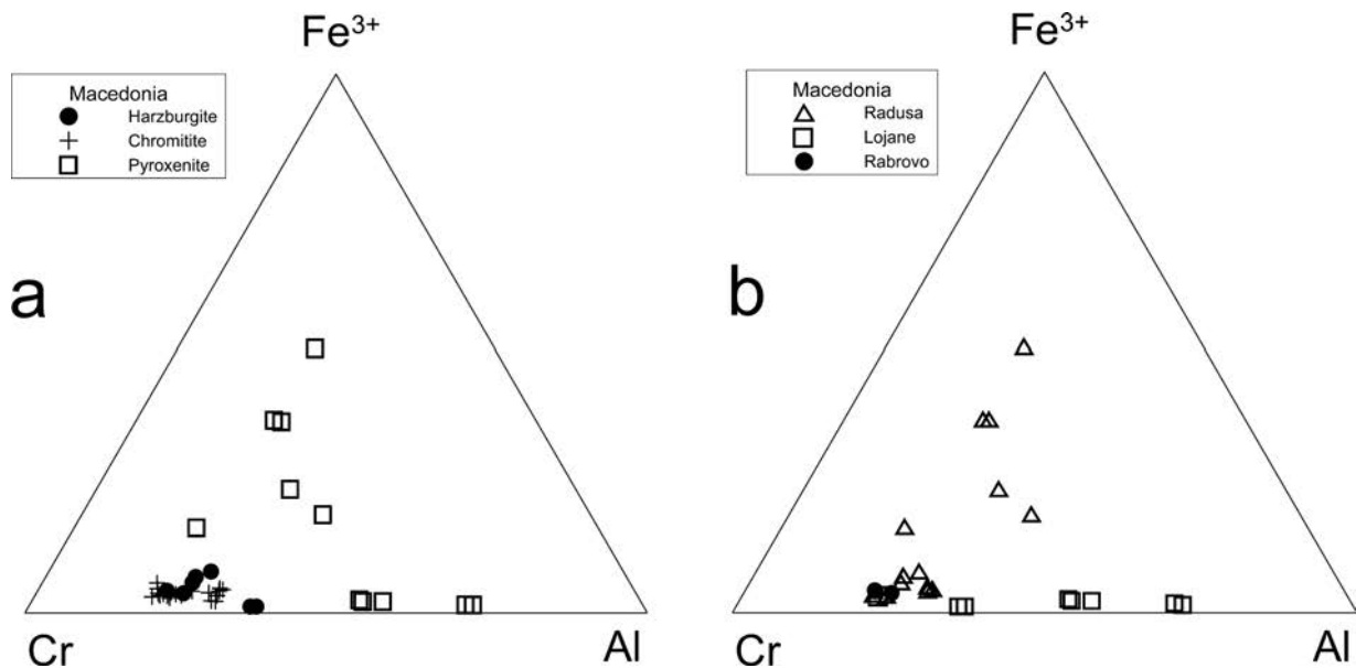
Fig. 6. Composition of chromite in the Cr–Al–Fe 3+ ternary diagram (a) by rock type and (b) by geological complex.
