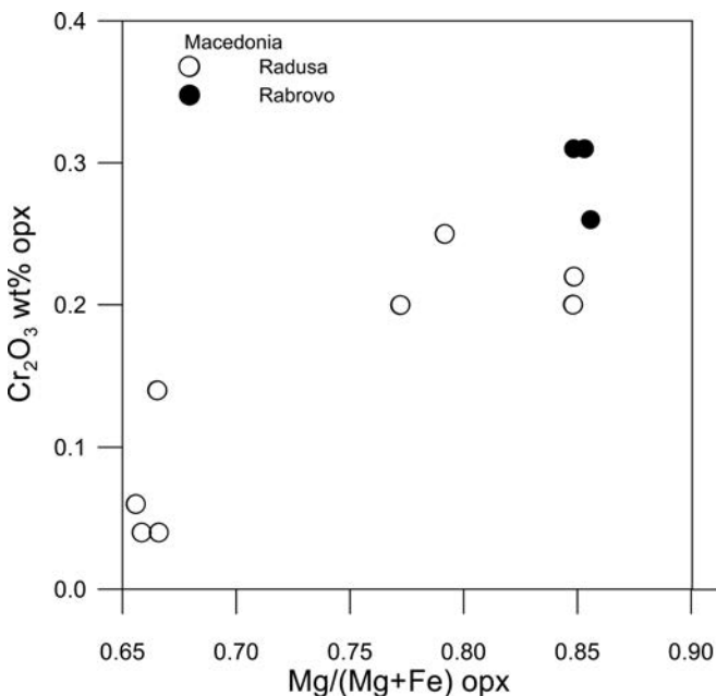
Fig. 3. Plot of Cr 2 O 3 vs. Mg/(Mg+Fe 2+ ) in molar percent in orthopyroxene for the Radusa and Rabrovo pyroxenites. This illustrates the differentiation trends in the Rabrovo pyroxenite.
