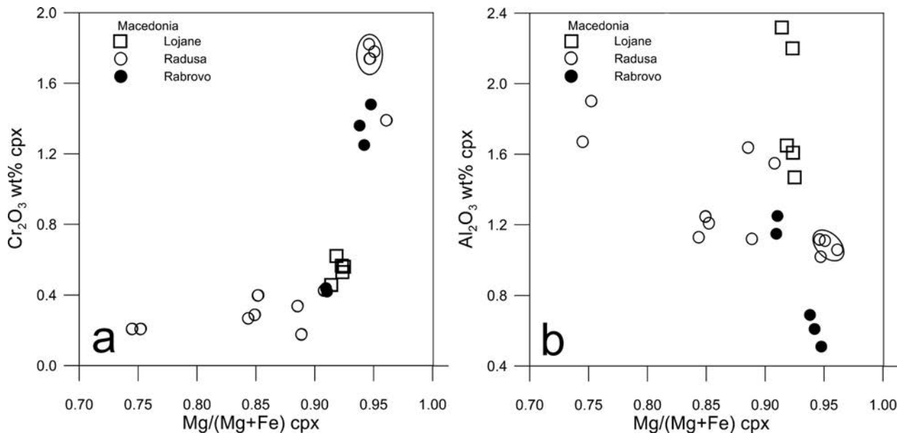
Fig. 4. Plots of (a) \text{Cr}_2\text{O}_3 vs. \text{Mg}/(\text{Mg}+\text{Fe}^{2+}) in molar percent and (b) \text{Al}_2\text{O}_3 vs. \text{Mg}/(\text{Mg}+\text{Fe}^{2+}) in molar percent in clinopyroxene for the Lojane, Radusa and Rabrovo pyroxenites. Minerals included in chromite are circled.
