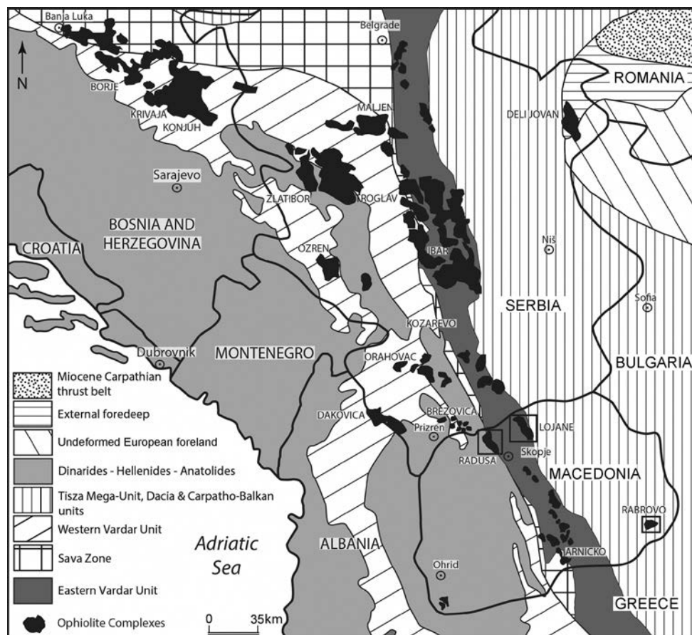
Fig. 1. Simplified geological map of the Eastern Mediterranean showing the principal ophiolite occurrences (after Bozovic et al. , 2013). Square: position of the three ophiolites studied in Macedonia.
