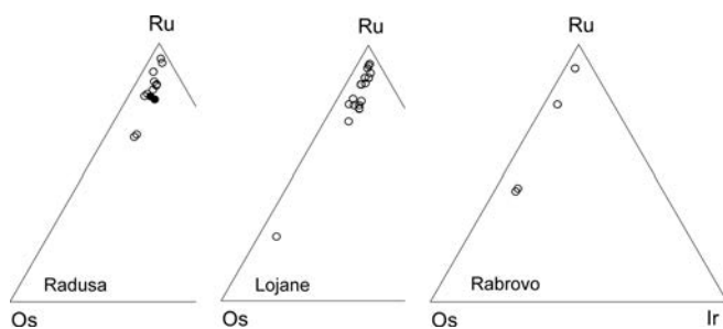
Fig. 10. Plots of Ru–Os sulfides (open circle) and alloy (black circle) in PGM included in chromite from chromite in the Lojane, Radusa and Rabrovo ophiolite complexes.
