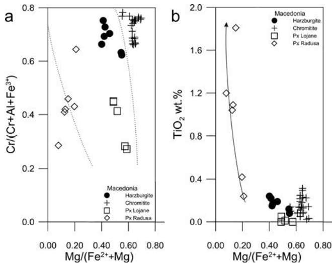
Fig. 7. Plots of (a) \text{Cr}/(\text{Cr}+\text{Al}+\text{Fe}^{3+}) vs. \text{Mg}/(\text{Mg}+\text{Fe}^{2+}) , both in molar percent (ophiolite domain, chromitite excluded, after Barnes & Roeder, 2001) and (b) wt% \text{TiO}_2 vs. \text{Mg}/(\text{Mg}+\text{Fe}^{2+}) in molar percent in chromite for chromitite, harzburgite and pyroxenite ( s.l. ) in the Macedonian ophiolite. The arrow shows the differentiation trends in the Radusa pyroxenite.
