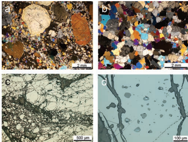
Fig. 2. Textures of selected rocks (a) porphyroblastic websterite, sample 57-5, Radusa Complex, Vitina Padina locality. (b) Pyroxenite, sample Ra1, adcumulate texture, Rabrovo Complex. (c) Submassive chromitite showing mylonite bands, sample 57-2 Radusa Complex, Vitina Padina ore body. (d) Cluster of silicate inclusions in a chromite crystal. Sample 41-5, Lojane chromitite. (a and b) cross-polarized transmitted light, (c and d) plane-polarized reflected light. Scale bar: (a), (b) 2 mm, (c) 0.5 mm, (d) 0.1 mm. (Online version in color.)
