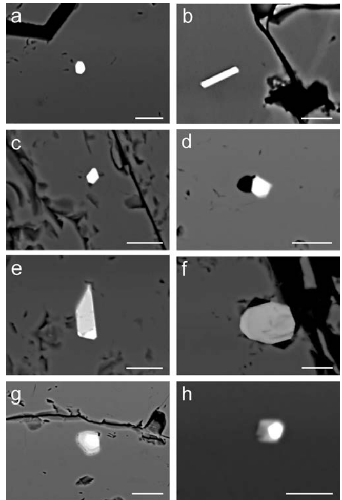
Fig. 8. Back-scattered electron images of PGM in chromite. (a) Euhedral laurite, sample 45-1, point 34 (Table 3). (b) Tabular laurite, sample 41-3. (c) Hexagon-shaped laurite, sample 42-1, point 21 (Table 3). (d) Euhedral laurite with an attached silicate (black), sample RaCr1b, point 14 (Table 3). (e) Polyphase inclusion, sample 44-1-b, with laurite (point 24, Table 3) – cuprorhodsite (point 27, Table 3). (f) Apparently altered laurite sample 41-1-b, point 32 (Table 3). (g) Laurite surrounded by a halo of an undetermined Cu sulfide. Sample RaCr1-a, point 10 (Table 3). (h) Laurite associated with an undetermined Cu mineral. Sample 44-1-c (point 29, Table 3). Scale bar is 10 \mu\text{m} .
