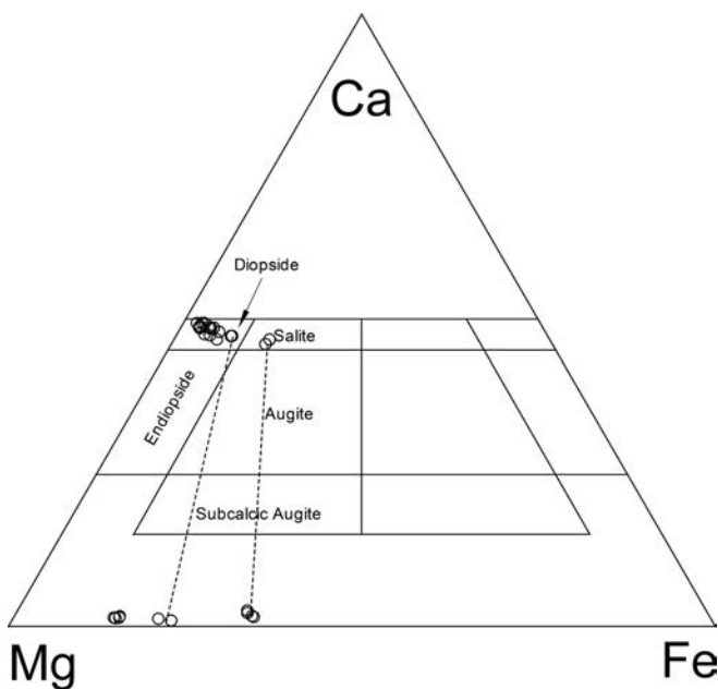
Fig. 5. Composition of ortho- and clinopyroxene in the pyroxene ternary diagram.
