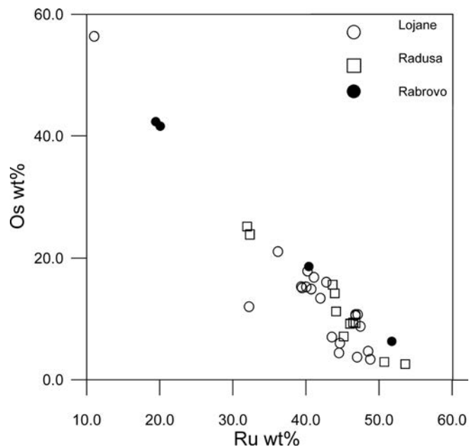
Fig. 9. Plot of Os vs. Ru in wt% in laurite included in chromite from chromite in the Lojane, Radusa and Rabrovo ophiolite complexes.
