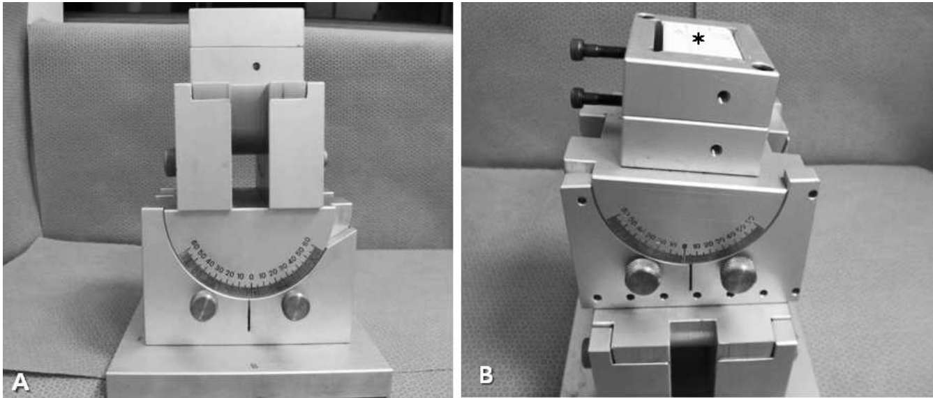
Figure 6. (A) Custom-designed and custom-manufactured surveyor system with rotational ability in all three planes. (B) Surgical stent (*) placed in the surveyor system. By using the custom-designed surveyor and a CNC machine, a guide hole was drilled in the surgical stent template according to the prescription angles measured on the cone-beam computed tomography data.
