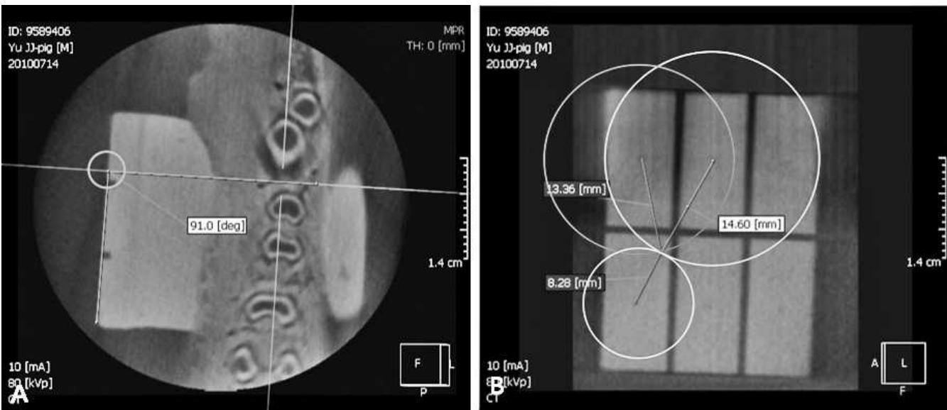
Figure 3. (A) The insertion point position for proper orthodontic mini-implant implantation was identified using image slices from cone-beam computed tomography data. (B) On the lateral flat surface of the surgical stent template, linear distances were measured from the insertion point to the three closest indentation holes. This information can be transferred to the physical Teflon-Perfluoroalkoxy surgical guide template by drawing the same circles on the stent using the correlative indentation holes as centers. The intersection of all three circles effectively reproduces the insertion point identified on the computer.
