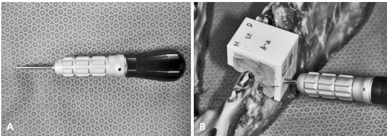
Figure 7. (A) A 1.5-mm-diameter hand drill (drill nose diameter = 2.5 mm). The drill nose diameter is the same as the orthodontic mini-implant (OMI) driver tip. (B) Cone-beam computed tomography-guided surgical stent used to insert a 1.5-mm OMI with a hand drill.
