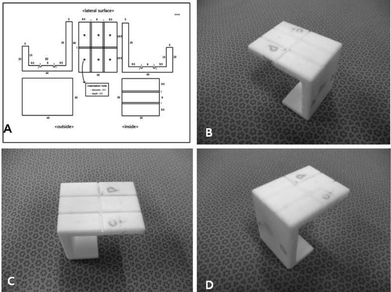
Figure 1. (A) Template for newly developed cone-beam computed tomography–assisted surgical stent for orthodontic mini-implant placement (numerical values are linear measurements in millimeters). (B–D) Actual surgical guide stent.
