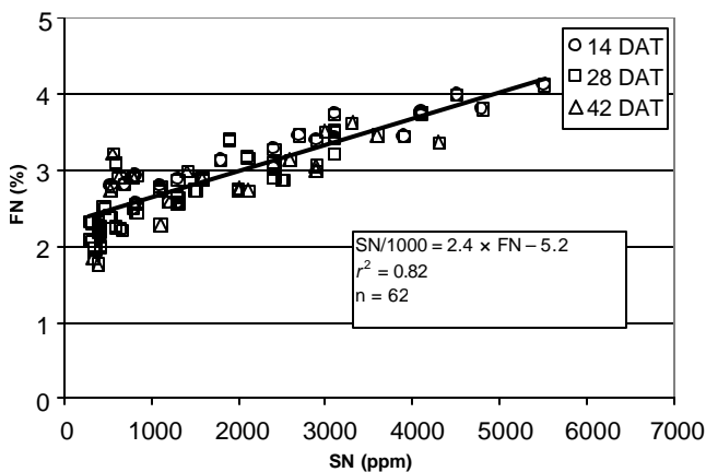
Fig. 1. Relationship between foliar nitrogen (FN) and petiole sap nitrate concentration (SN) of 'Pacifica White' vinca harvested at three dates (Exp. 1).
