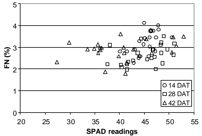
Fig. 2. Relationship between foliar nitrogen (FN) and SPAD readings of ‘Pacifica White’ vinca (Expt. 1).
