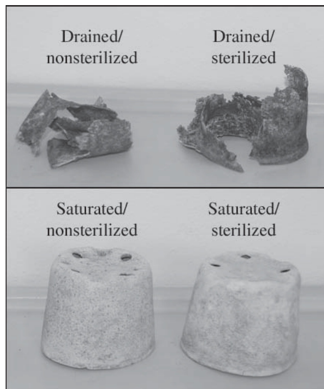
Fig. 2. Representative bioplastic containers placed in saturated soil (bottom) were intact and, though misshapen, retained their original form at the end of the second experiment. In contrast, containers placed in drained soil (top) degraded extensively and lost structural integrity. Prior sterilization of media in the containers and of the soil in which the containers were planted did not influence weight loss of the containers, which was used to quantify degradation.
