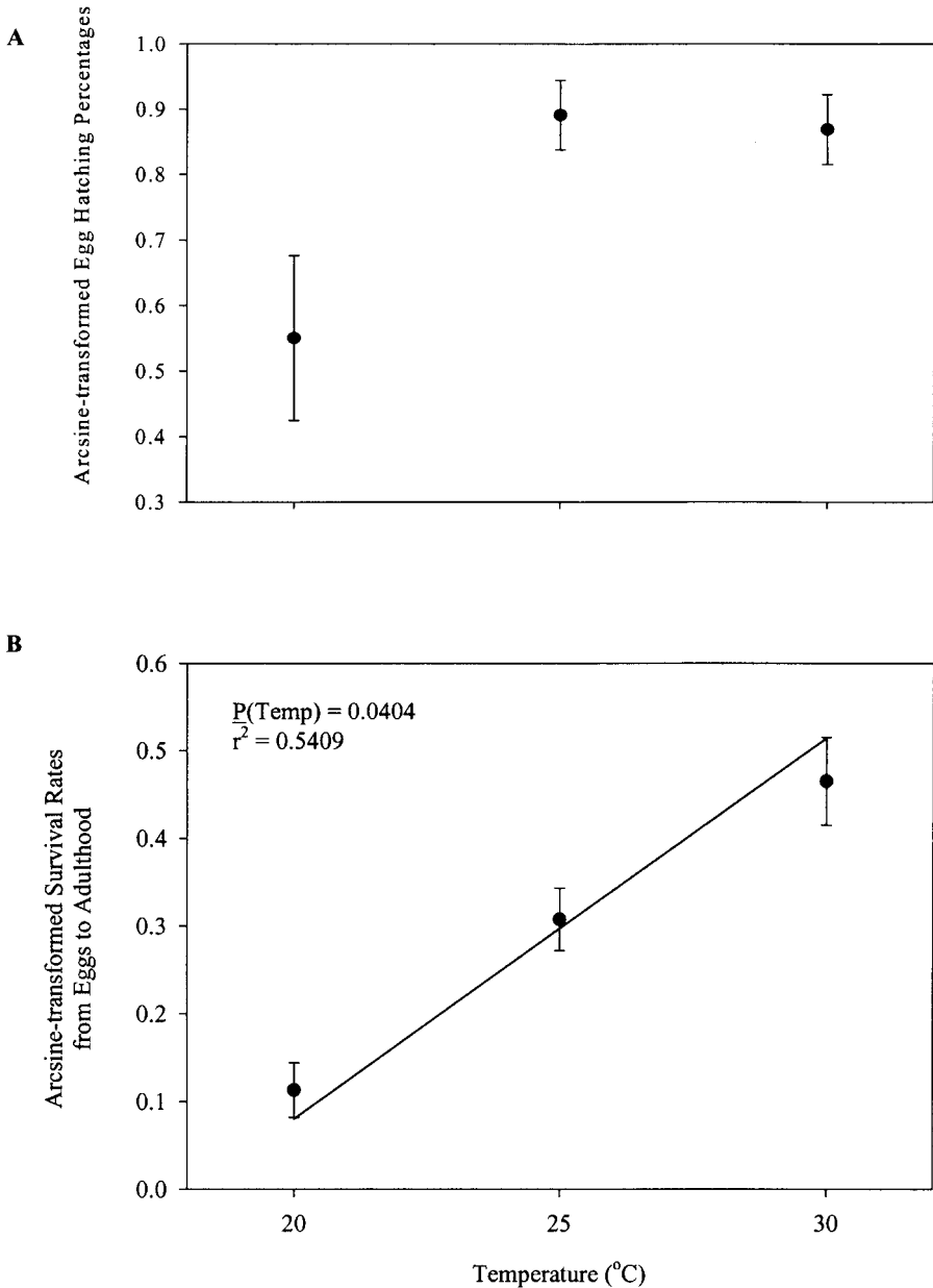
Fig. 2. Arcsine-transformed mean ( \pm SE) egg eclosion percentage (A) and survival rate to adulthood (B) of P. madeirensis at the three temperatures. The main effects of CO 2 and generations were not significant. Line represents the result of linear regression analysis. P-value presented is that of the temperature treatment.
