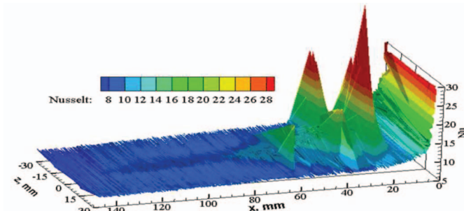
Computed local Nusselt number distribution
