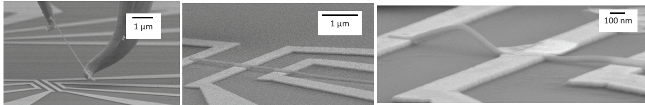
Figure 2. Nanowires are moved to pre-fabricated devices made with electron beam lithography. Images show a nanowire before and after junctions are welded.
