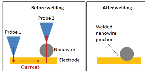
Figure 2. Nanowires are moved to pre-fabricated devices made with electron beam lithography. Images show a nanowire before and after junctions are welded.
