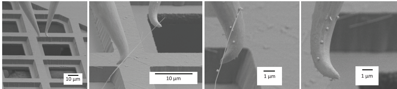
Figure 1. Probes are used to lift nanowire off metal grid and pass current through the wire. Contact resistance between probe and nanowire leads to local melting resulting in solder-like balls.
