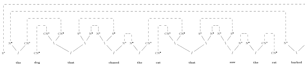
Figure 3 Proof net analysis of (4b) the dog that chased the cat that saw the rat barked .
