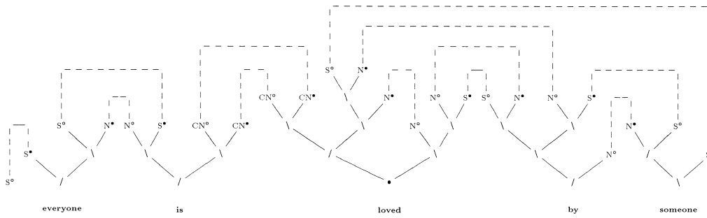
Figure 9 Proof net analysis for the subject wide scope reading of (7b) everyone is loved by someone ( \forall\exists ).
