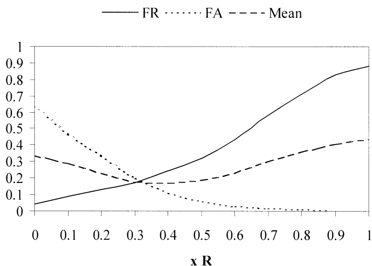
Figure 8 FR, FA, and mean error for group A related to threshold values expressed as subdivisions of R .
