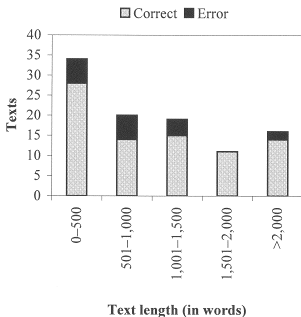
Figure 4 Text length related to accuracy for the text genre detection experiment.
