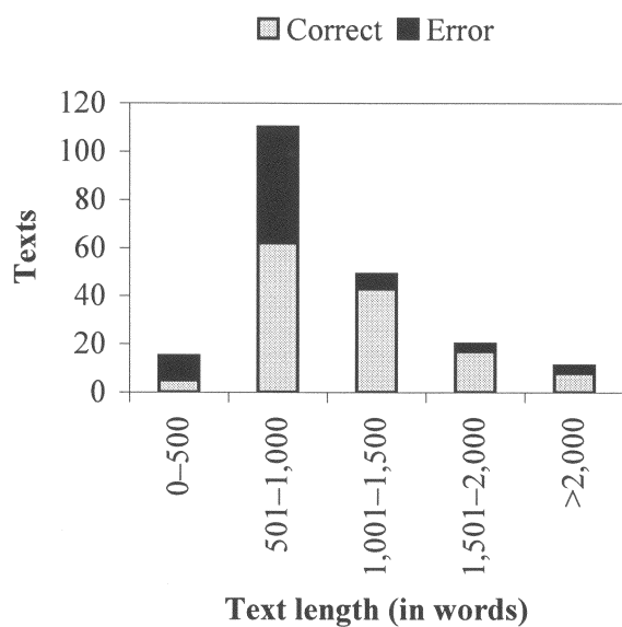
Figure 7 Text length related to accuracy for the author identification experiments.
