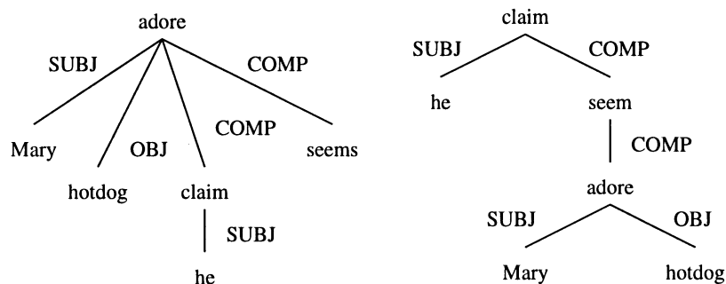
Figure 25 LTAG derivation tree for (14) (left); dependency tree for (14) (right).
