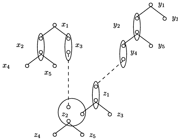
Figure 9 Derivation of an elementary d-tree.
