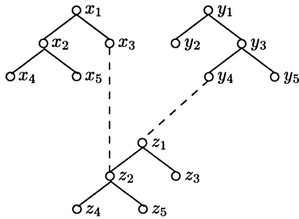
Figure 6 A tree description (which is also a d-tree) with three components.
