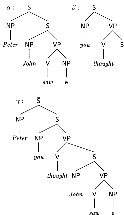
Figure 1 Example of adjunction.
