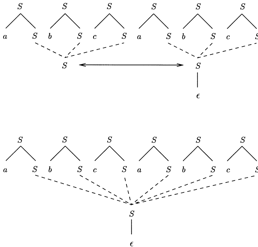
Figure 13 A grammar for Mix.
