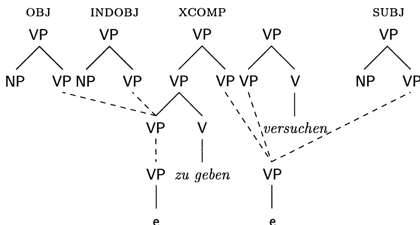
Figure 24 DSG derivation for a complex sentence.
