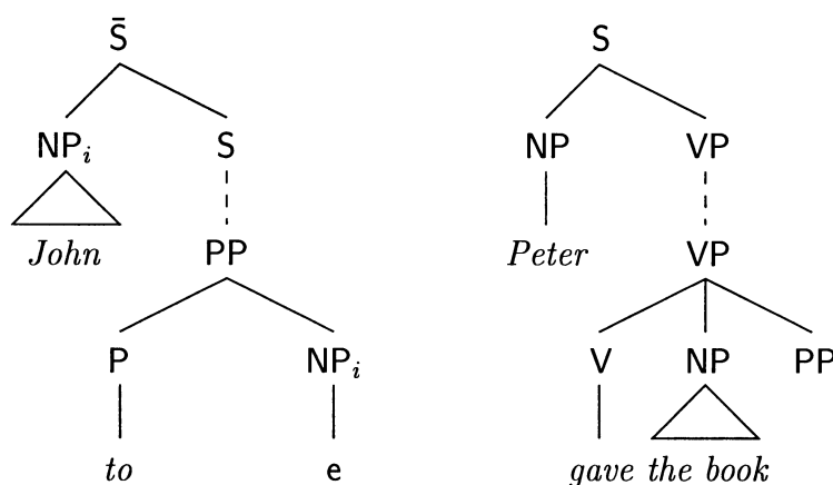
Figure 15 HPSG analysis of give expressed as trees.
