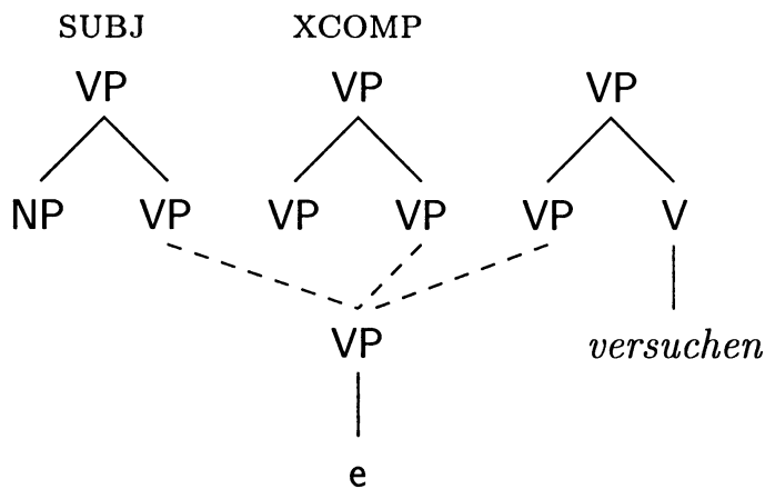
Figure 23 D-tree for German verb versuchen 'to try'.
