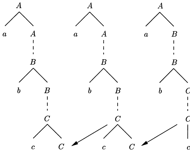
Figure 11 Counting to three: A derivation.
