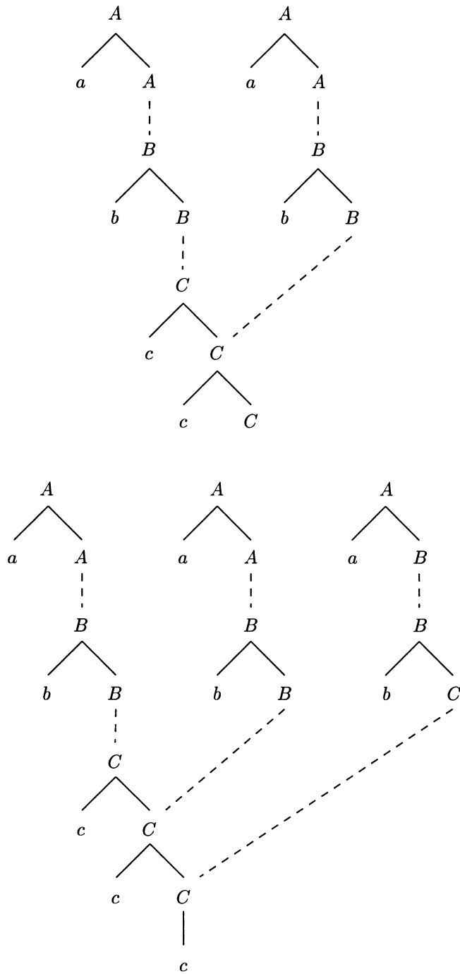
Figure 12 Counting to three: After substituting one tree (above) and the derived d-tree (below).
