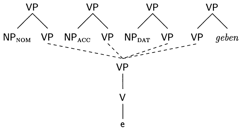
Figure 22 D-tree for German verb geben 'to give'.
