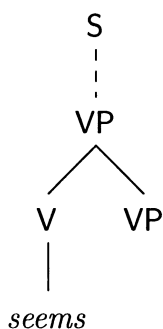
Figure 26 Elementary d-tree for finite seems .
