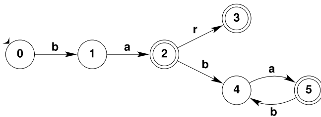
Figure 4 Minimal automaton accepting the set of strings (ba)^+ \cup \{\text{bar}\} .
