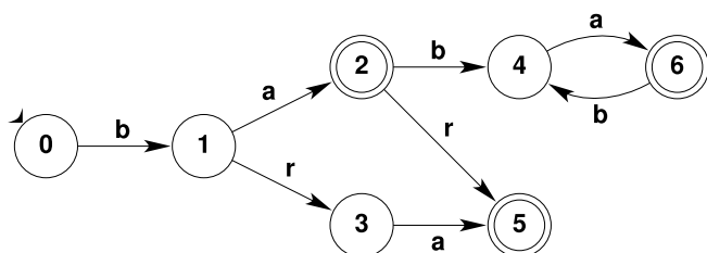
Figure 7 Minimal automaton accepting the set (ba)^+ \cup \{\text{bar}\} \cup \{\text{bra}\} .
