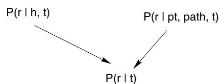
Figure 9 Minimal lattice.
