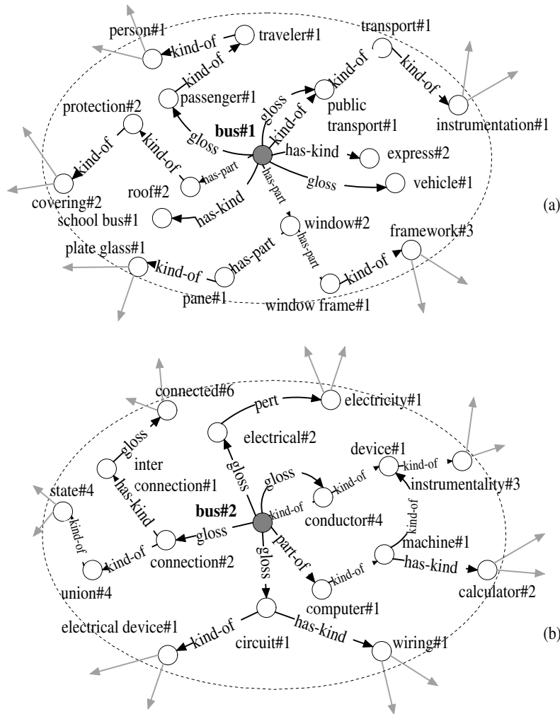
Figure 7 Graph representations for (a) sense 1 and (b) sense 2 of bus.
