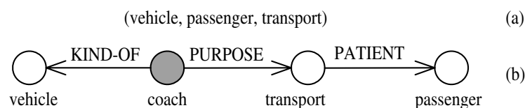
Figure 6 Two representations of the same concept: (a) as a feature vector and (b) as a semantic graph.
