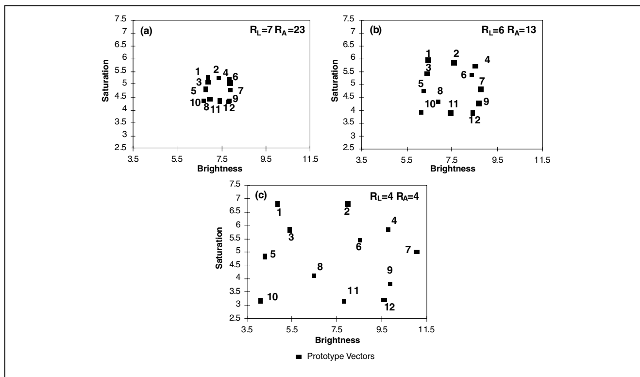
Figure 6. Spatial organization of the prototype population vectors during training. The figure depicts the population encoding representations of the prototype vectors in the brightness/saturation feature space (solid squares). Time (training) progresses from subfigure (a) to (c).
