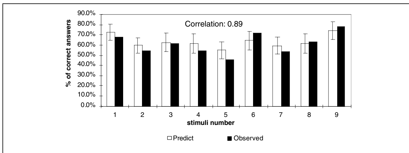
Figure 3. Comparison of predicted vs. observed correct identification frequencies (diagonal values) for all nine stimuli in the Shepard's identification task. Black bars represent the percentage of correct answers in human data, and white bars represent the model generated responses. The standard error of the model responses is portrayed by the error bar on top of the model white bars.
