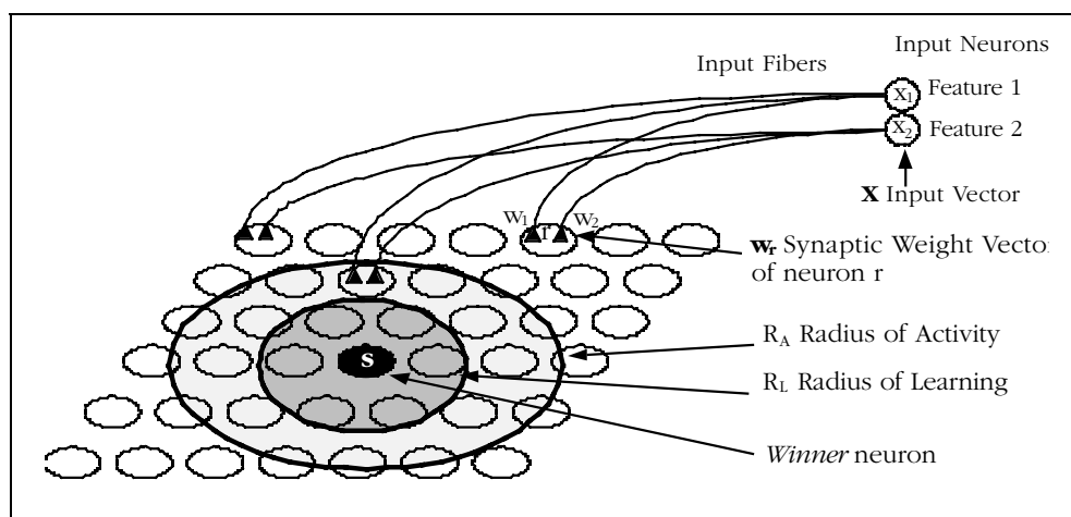
Figure 1. Schematic model description. The neural model is composed of a two-dimensional array of neurons fully connected to a common source of input fibers transmitting the input stimuli.
