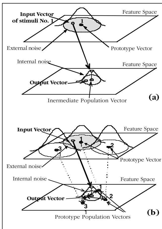
Figure 2. Reading the network's output. The figure demonstrates the identification process. (a) An input vector is chosen from a normal distribution (simulating external noise) centered around a prototype feature vector stimulus (e.g., stimulus No. 1). The network processing assigns an intermediate population vector to the input vector in the feature space. The final output vector is determined by adding a normal distribution noise term to the population vector, simulating internal noise factors in human processing. (b) The output response is then identified by finding which of the prototype population vectors is the closest to the output vector in the new mapping.
