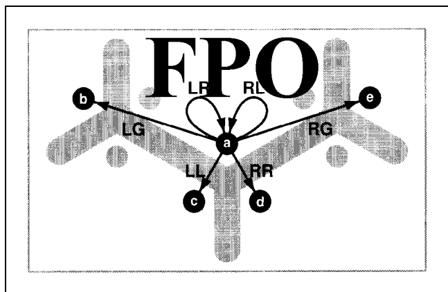
Figure 12. Possible movement decisions when facing the view marked a . L: turn left 60°. R: turn right 60°. G: go ahead to next place.
