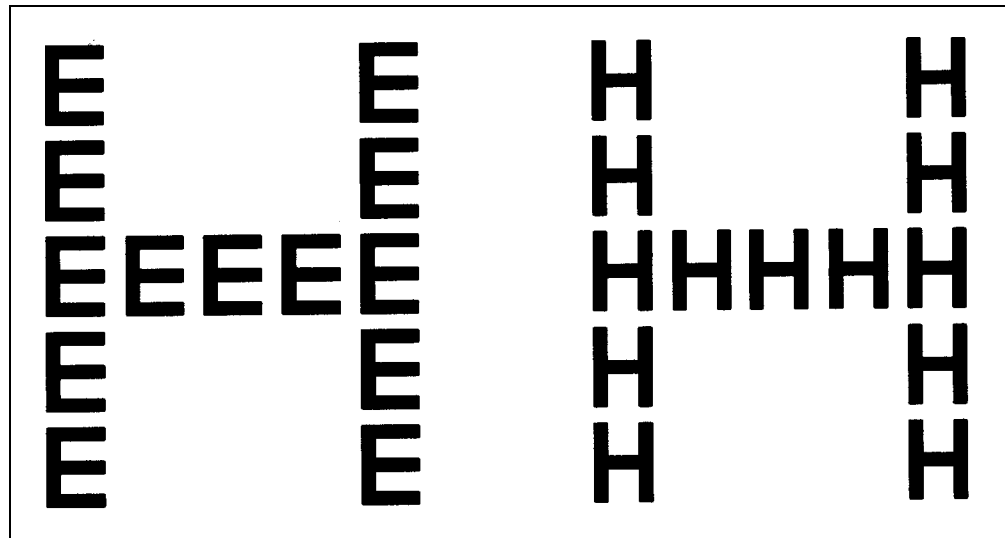
Figure 1. Examples of the stimuli used in this study. Left, the letter H is formed at the global level by the letters E at the local level. The global and local letters could either be different (left of figure) or the same. In the study, only one hierarchical letter was presented on each trial. A fixation spot (not shown) was present in the center of the display, and a frame surrounded the locations at which the letters would be flashed. Both the letters and frame were actually presented white on a black background.
