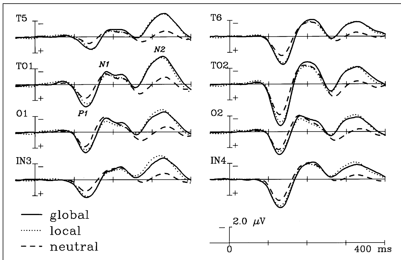
Figure 4. Grand average ERPs across the 10 subjects in the selective attention task. The ERPs (plotted negative polarity upward) are shown for left and right posterior temporal (T5, T6), lateral occipital (TO1, TO2), occipital (O1, O2), and inferior occipital (IN3, IN4) scalp sites. Stimulus onset is at the vertical calibration bar, and tick marks indicate 100-msec intervals. The P1 and N2 components are labeled at the TO1 sites but can be observed at all these posterior sites.
