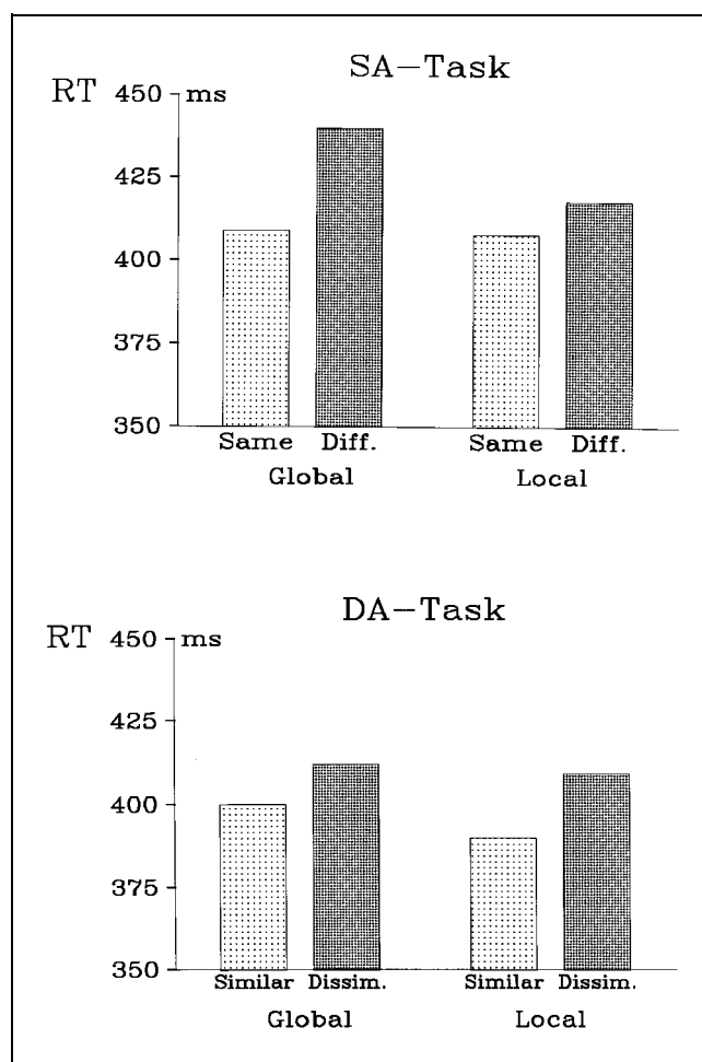
Figure 2. Mean reaction times to target letters in the selective-attention (SA) task (top) and divided-attention (DA) task (bottom). In the SA task, letters at the global and local levels could be the same or different. In the DA task, letters at the global and local levels could be similar in form (letters S and E) or dissimilar in form (letters H and A) and could appear at either the global or local level.
