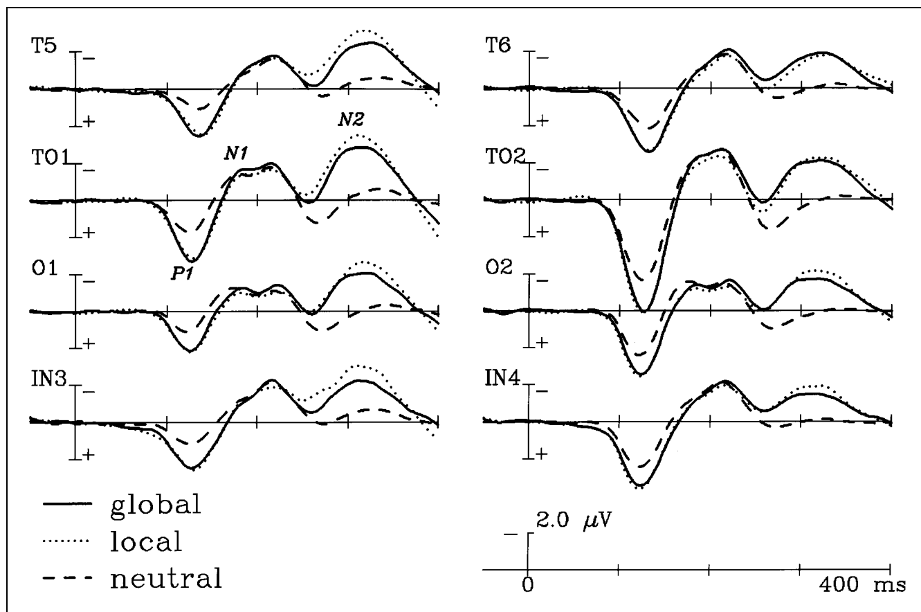
Figure 7. Grand average ERPs across the 10 subjects in the divided-attention condition. Differences in the N2 elicited by target stimuli can be seen over the left hemisphere (left column) and right hemisphere (right column). In particular, the N2 to local targets (dotted line) was greater in amplitude than the N2 to global targets (solid line) over the left hemisphere (T5 and T01 sites in particular), but over the right hemisphere, the N2 to global and local targets are more similar in amplitude.
