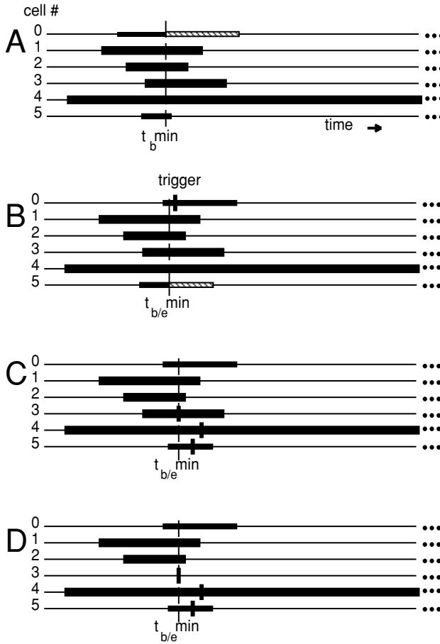
Figure 2: Typical sequence of local integration steps in a six-cell example. The t_a to t_b intervals of possible interpolation are shown as black rectangles. The t_{b/e}^{\min} is shown as a vertical dashed line. (A) Integration coordinator requests integration for lagging cell (# 0 with minimum t_b ). Integrator advances by dt (length of hashed rectangle). In that step, we suppose cell 0 crosses the threshold, and a threshold event is generated, labeled "trigger" in panel B. This is an event whose time is tentative since unprocessed synaptic events could still influence this cell. (B) Cell 5 has minimum t_b and integrates forward. (C) The trigger event is at t_{b/e}^{\min} . The handling of this trigger creates three events to be delivered to cells 3,4,5 at varying delays (short vertical lines). We suppose that its delay places the cell 3 input event earlier than any t_b . (D) The event in cell 3 is now t_{b/e}^{\min} . Cell 3 back-interpolates, the event is handled, and cell 3 reinitializes, giving t_a^3 = t_b^3 = t_{b/e}^{\min} . Cell 3 will be the next cell to integrate forward.
