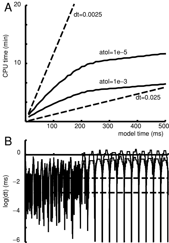
Figure 4: Comparison of fixed and variable time-step methods for the mutual-inhibition model. (A) CPU time increases linearly with simulation time for fixed-step method (dashed lines for dt = 2.5\mu\text{s} – upper curve; dt = 25\mu\text{s} – lower). There is a reduction in CPU load at the onset of synchrony using the variable-step method (solid lines with absolute error tolerance 1 \cdot 10^{-5} – upper; 1 \cdot 10^{-3} – lower). (B) Time-step size as a function of time. \text{Log}(dt) is shown for fixed dt (horizontal dashed lines) and variable dt in one neuron (solid lines).
