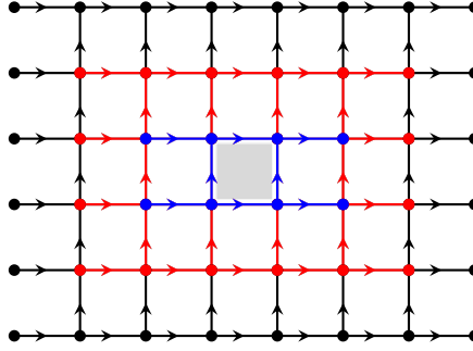
FIG. 2. The patch graph P_6 contains P_4 (in red and blue) and P_2 (in blue) as subgraphs which share the same center plaquette, shown in gray. We define a distance function d(e) on the edges e of P_n , which takes integer values between 1 and n/2 . In this example the black edges are those with d(e)=3 , the red edges have d(e)=2 , and the blue edges have d(e)=1 .
