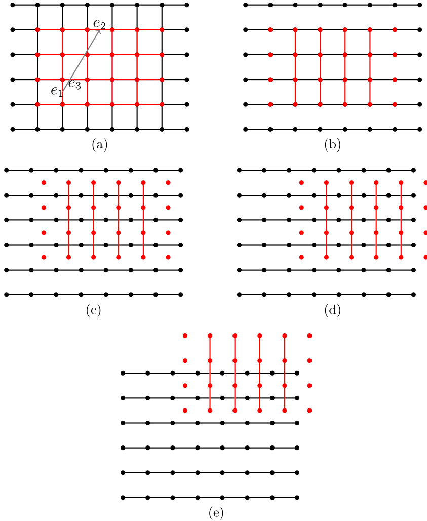
FIG. 4. Here we take n = 3 , j = 2 , and j' = 3 and we illustrate how to compute R_{j,j'}(e_1, e_2) , where the edges e_1, e_2 , and e_3 are shown in (a). We start with overlapping cocentered copies of P_{2j} (red in (a)) and P_{2j'} (red and black in (a)). Although these are directed graphs we have not drawn the edge orientations since they are irrelevant here. Form new graphs \tilde{P}_{2j} and \tilde{P}_{2j'} , shown in (b), by retaining only the edges which are parallel to e_1 and e_2 , respectively. Then apply the shift T_{e_1 \rightarrow e_2} to \tilde{P}_{2j} (shown in (c)); then R_{j,j'}(e_1, e_2) = 8 is the number of edge midpoints which overlap between this graph and \tilde{P}_{2j'} . We can decompose the shift as T_{e_1 \rightarrow e_2} = T_v T_h T_{e_1 \rightarrow e_3} where T_v and T_h are vertical and horizontal translations, respectively. Subfigures (c) and (d) show \tilde{P}_{2j'} along with T_{e_1 \rightarrow e_3}(\tilde{P}_{2j}) and T_h T_{e_1 \rightarrow e_3}(\tilde{P}_{2j}) , respectively.
