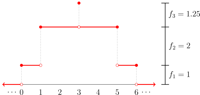
FIG. 3. We extend \{c_1, \dots, c_{n-2}\} to a function c(x) on \mathbb{R} . Here we show an example with n = 8 and \{c_0, c_1, c_2, c_3, c_4, c_5, c_6\} = \{1, 3, 3, 4.25, 3, 3, 1\} .
