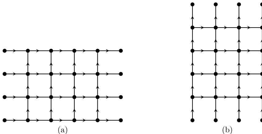
FIG. 1. Directed graphs P_n and Q_n for n = 4 .
