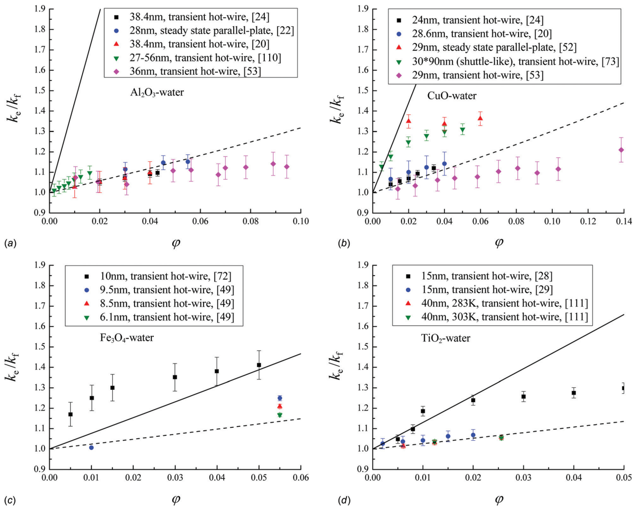
Fig. 6 Comparison between experimental data and H-S bounds (solid line: H-S upper bound; dash line: H-S lower bound)
