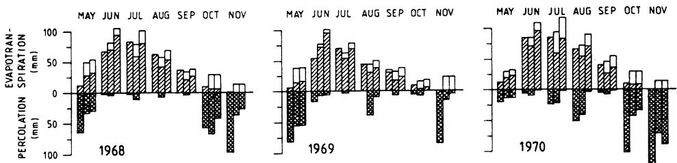
Fig. 5. Simulated interception (unfilled) and transpiration (dashed mm/month). From left to right: Sjöängen 6 (grassland), Sjöängen 7 and 8 (forest). Chequered columns show percolation (mm/month).
