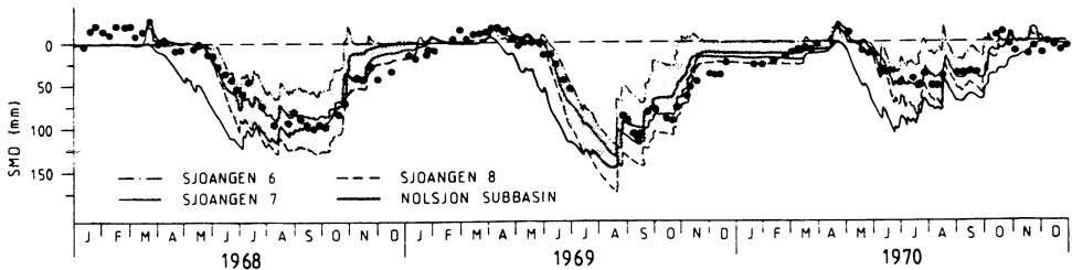
Fig. 4. Measured and simulated soil moisture deficits. Simulated with the SM-model for the forest stations 7 and 8 at Sjöängen and with the PULSE-runoff model for the Nolsjön subbasin as a whole. Measurements (points) refer to station 7 (where the most frequent measurements took place). The PULSE model simulation is discussed in the section »Groundwater Recharge Regime and Runoff Formation Process«.
