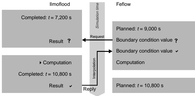
Figure 7 | Procedure of the request-reply mechanism for the uni-directional connection between Ilmflood and Feflow.
