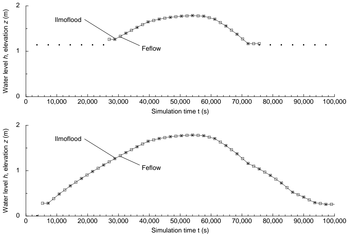
Figure 8 | Results of the Ilmflood model (water level or elevation in case of dry cell) and adjacent boundary conditions set in the Feflow model for the links between cell 20 and node 112 (top) and cell 8 and node 17 (bottom).
