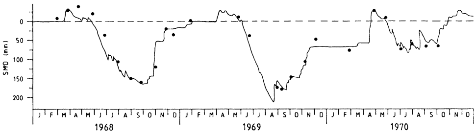
Fig. 7. Measured (points) and simulated soil moisture deficits at Spekeläggen before deforestation (1968-1970). All available soil moisture data were used for the parameter optimization.
