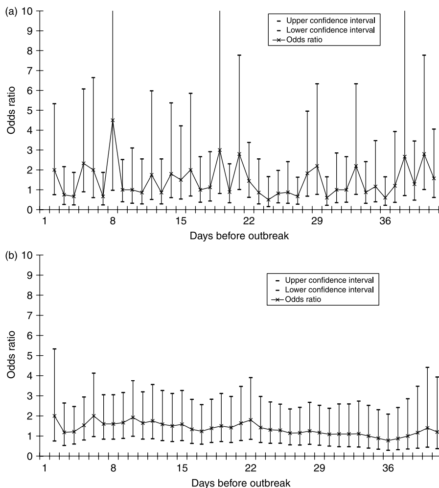
Figure 2 | Estimated odds ratios and their 95% confidence intervals for exceedance event by day before outbreak. (Second method) (a) matched comparison of case and control years. (b) cumulative exceedance based on matched case and control pairs.
