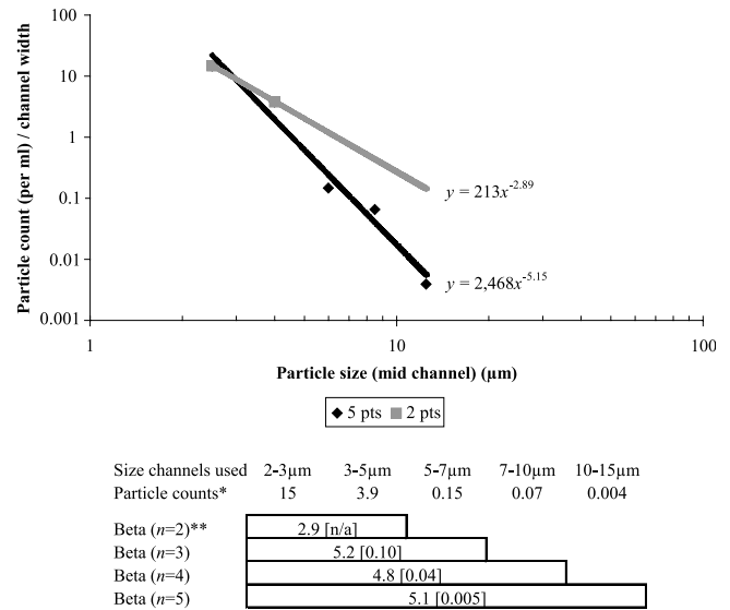
Figure 3 | Beta estimates calculated using different size channels (light obscuration sensor, filtered groundwater sample). *Normalised particle count (i.e. divided through by channel width). **n=number of indicated size channels used to calculate beta. The significance level [P] associated with each β calculation is shown in square brackets.
