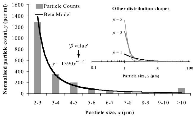
Figure 1 | Typical size distribution of particles in water.
