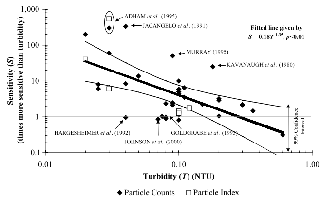
Figure 4 | Particle monitor sensitivity model (literature data).
