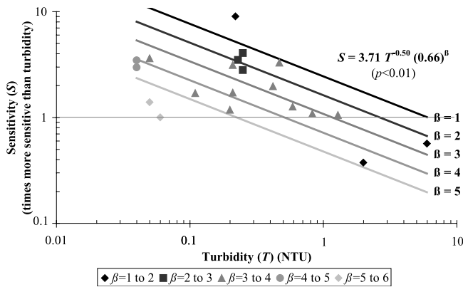
Figure 5 | Particle counter sensitivity model with \beta (experimental data).
