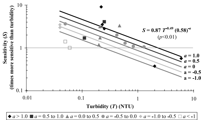
Figure 6 | Particle counter sensitivity model with particle ratio (experimental data).
