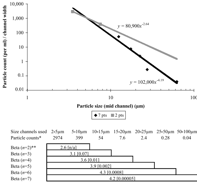
Figure 2 | Beta estimates calculated using different size channels (light obscuration sensor, surface water sample, data taken from Hargesheimer & Lewis 1995). *Normalised particle count (i.e. divided through by channel width). **n=number of indicated size channels used to calculate beta. The significance level [P] associated with each β calculation is shown in square brackets.
