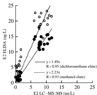
Figure 3 Comparison of analytical results between E2 ELISA and LC-MS/MS instrumental analysis for determination of E2 in STP. For E2 ELISA, the sample was extracted with SPE column (C18) and eluted with dichloromethane (●) or methanol (○)
