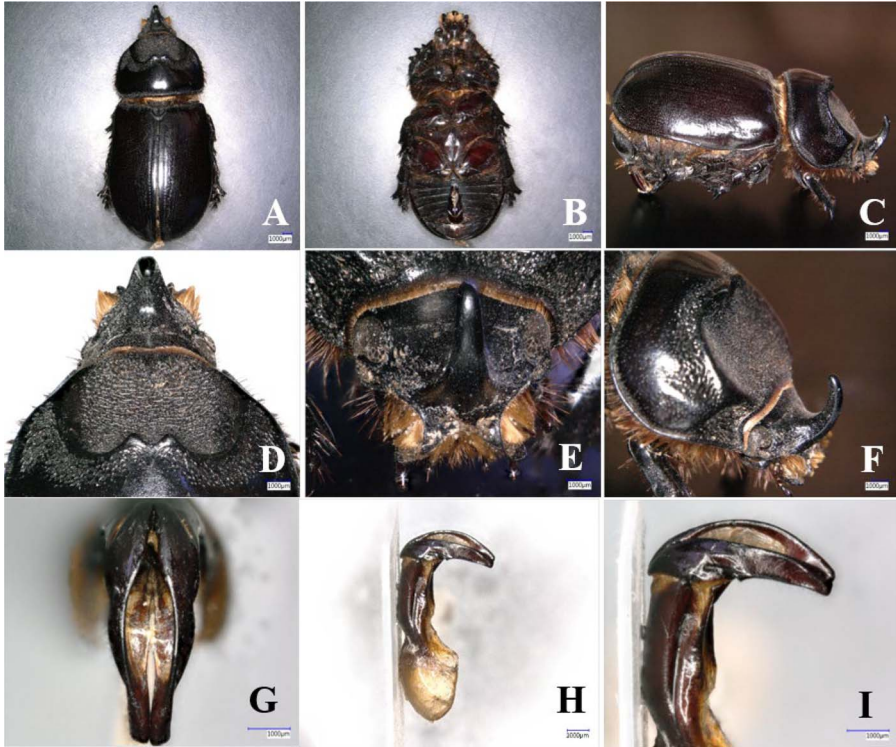
Fig. 2. Male Oryctes agamemnon arabicus dorsal view (A); ventral view (B); lateral view (C); head in dorsal view (D); head in frontal view (E); head in lateral view (F); paramera in caudal view (G); paramera in lateral view (H); paramera in lateral view (I).
