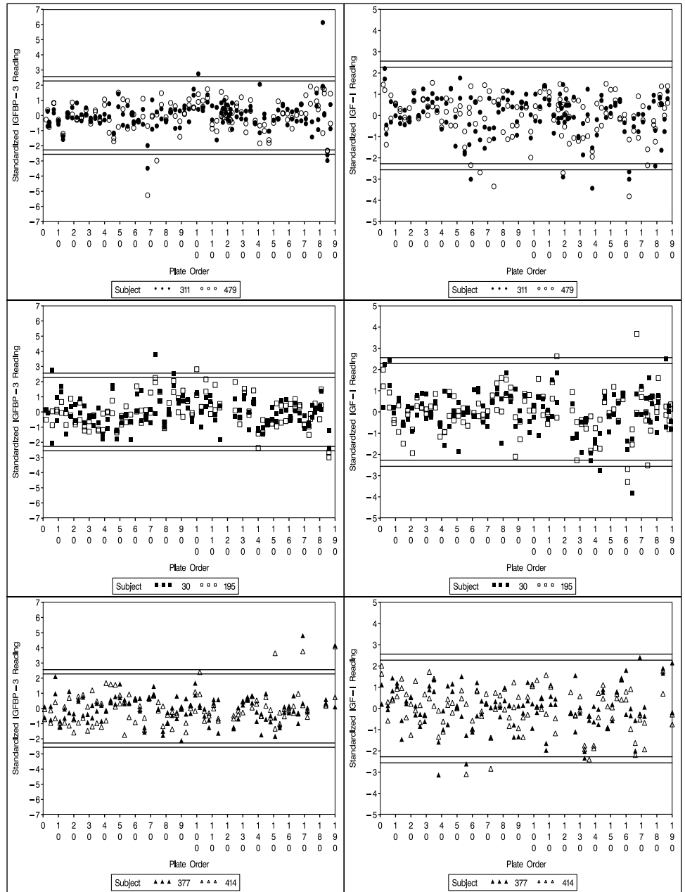
Figure 1. Modified Levy-Jennings plots for six QC subjects over 188 plates/batches for IGF-I and IGFBP-3 assays.
