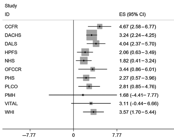
Figure 1. The association between the weighted genetic risk score (the instrumental variable) and BMI across the 11 participating studies in GECCO and C-CFR.
