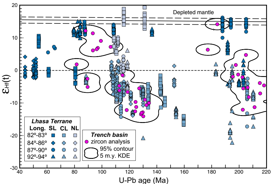
Figure 4. Paired detrital zircon Hf isotopic data and U-Pb ages from our Rongmawa Formation (southern Tibet) samples ( n = 50 ; pink circles) plotted on Hf evolution diagram and compared against Lhasa terrane reference data from Zhu et al. (2011) (blue symbols); 95% contour is shown for three-dimensional (3-D) kernel density estimate (KDE) surface with 5 m.y. x-axis bandwidth and 1 \epsilon_{\text{Hf}} y-axis bandwidth calculated from Rongmawa Formation data, created with HafniumPlotter (Sundell et al., 2019). Reference data are split into four longitudinal (Long.) swaths between 82°E and 94°E, shown by shades of blue, and by position within the Lhasa terrane, shown by different symbols. SL—southern Lhasa terrane; CL—central Lhasa terrane; NL—northern Lhasa terrane. Data were normalized to chondritic uniform reservoir (CHUR; dashed line at 0 \epsilon_{\text{Hf}} ). Depleted mantle isotopic composition is shown with 95% confidence intervals (solid line and long-dashed lines).
