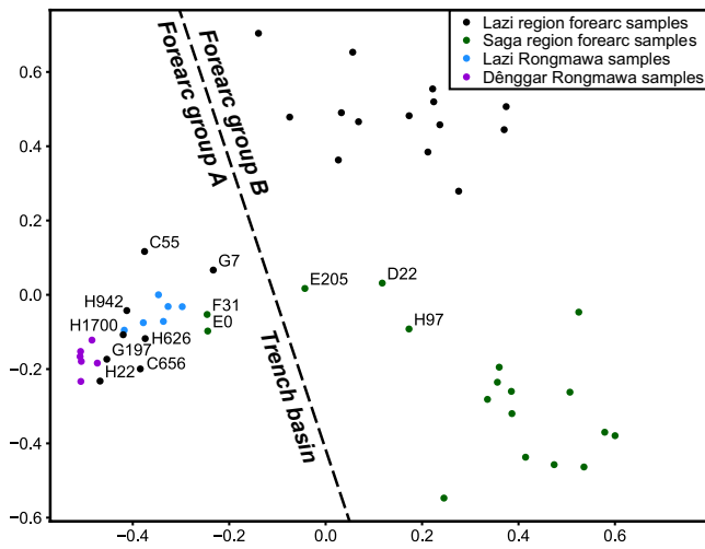
Figure 3. Multidimensional scaling (MDS; Vermeesch, 2013) results for all Xigaze Group forearc strata and Rongmawa Formation trench basin strata (southern Tibet), with interpreted boundary (dashed line) between samples displaying local Gangdese magmatic arc provenance and samples displaying distal, central Lhasa terrane provenance. Plot shows Kolmogorov-Smirnov dissimilarities between samples as a map where similar samples cluster and differing samples plot far apart. Sample names are provided for select forearc samples from Orme et al. (2015) and Orme and Laskowski (2016) that plot close to Rongmawa Formation samples.
