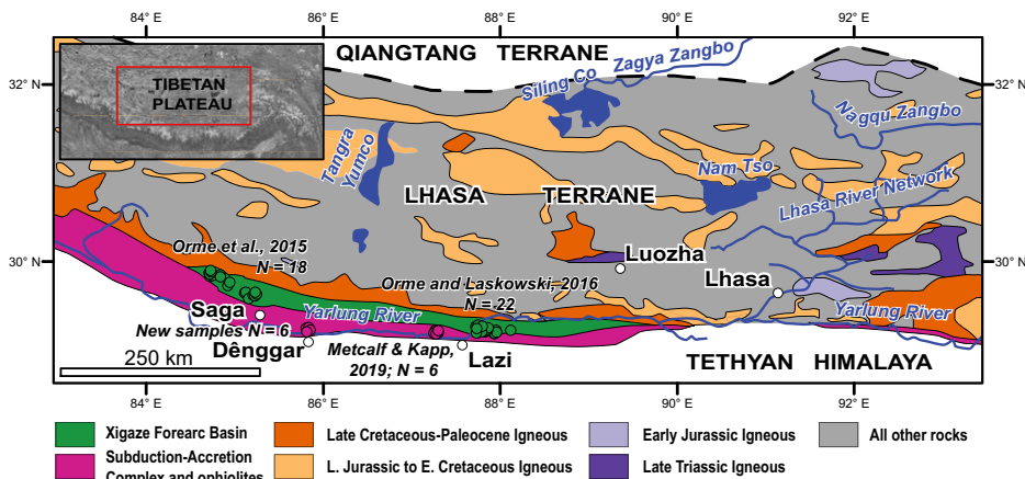
Figure 1. Tectonic map of the Lhasa terrane and Yarlung suture zone in south-central Tibet, modified from Zhu et al. (2011). Mesozoic and early Cenozoic igneous rocks of the Lhasa terrane are highlighted due to their importance for detrital zircon provenance analysis. Xigaze Group forearc basin sample locations are shown in green (Orme et al., 2015; Orme and Laskowski, 2016), whereas Rongmawa Formation (trench basin) samples are shown in pink (this study; Metcalf and Kapp, 2019). Major rivers and locations of towns were traced from the Esri World Topographic Map ( http://arcg.is/0r4aaH ).
