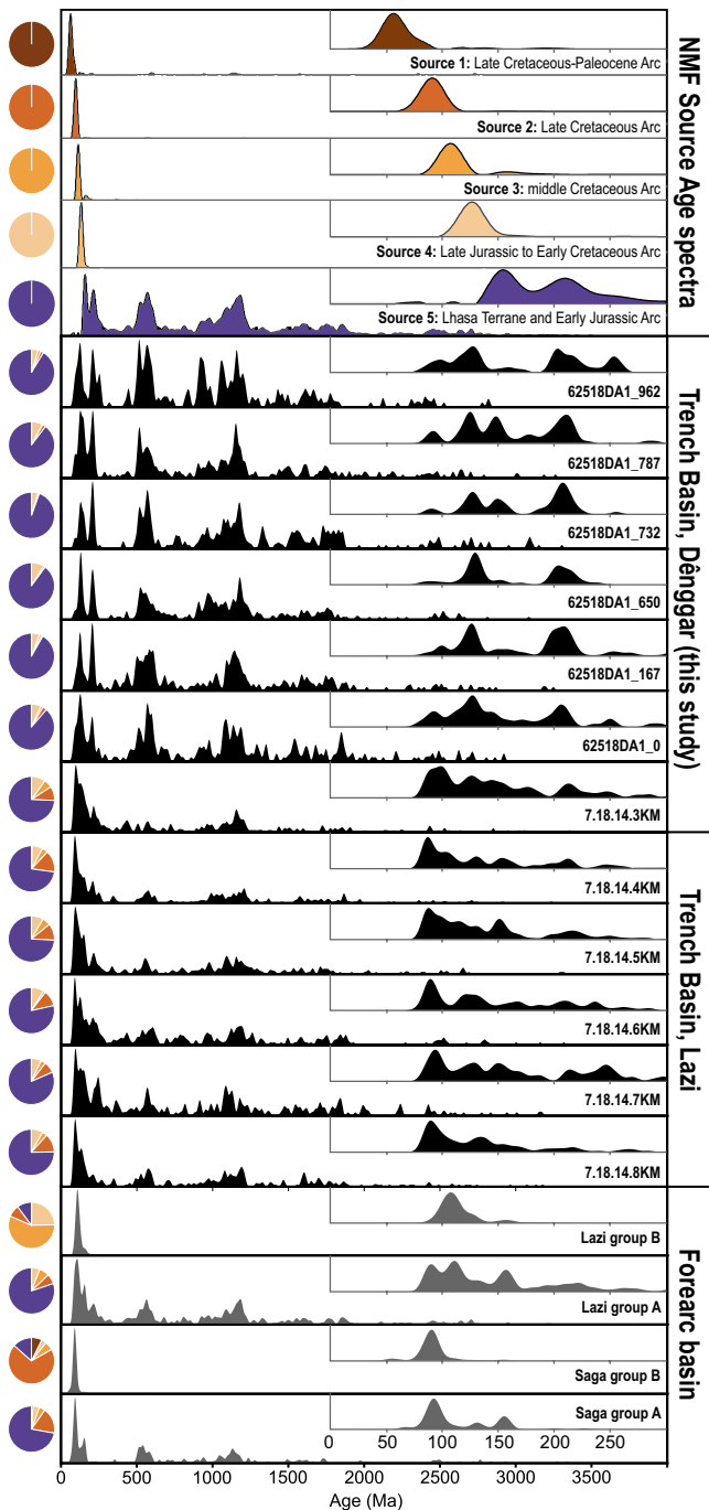
Figure 2. Non-normalized kernel density estimate (KDE) plots of individual Rongmawa Formation samples (black); composite KDEs of Xigaze Group forearc basin samples (gray) separated by geographic region (Fig. 1) and proximity to trench basin samples on MDS plot (Fig. 3); KDE representations of five optimal sources for all Rongmawa Formation and Xigaze Group forearc samples deconvolved using detrital zircon nonnegative matrix factorization (NMF; at top); and pie diagrams showing proportion of each NMF source in each age spectrum (at left, keyed by color). Spectra are plotted with relative probability on vertical axis, and U-Pb age between 0 and 4000 Ma on horizontal axis. Inset plot shows component of spectra between 0 and 300 Ma.
