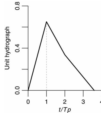
Figure 1 | Instantaneous unit hydrograph (IUH) of ReFH model.
