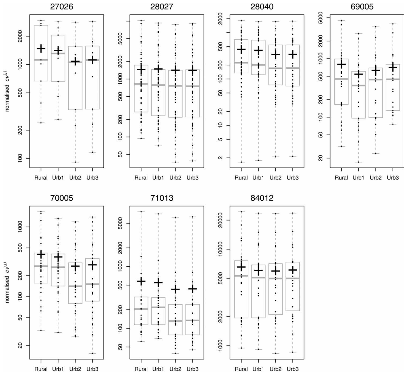
Figure 3 | Comparison of normalised cross-validation statistics ( \text{mm}^2 \text{h}^{-2} ) for individual events cv^{(i)} for all catchments and for all model variants. Box-plot shows the 75, 50 (median) and 25% quantiles, as well as the maximum and minimum values. The corresponding mean values are indicated with a + symbol.
