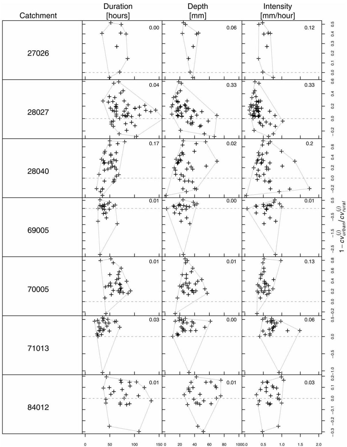
Figure 6 | Plot of relative cross-validation statistics (Equation (13), percentage improvement over original model) against storm characteristics (duration, depth and intensity) model Urban3. Number in upper right corner of each plot is the r^2 coefficient of determination value obtained through linear regression.
