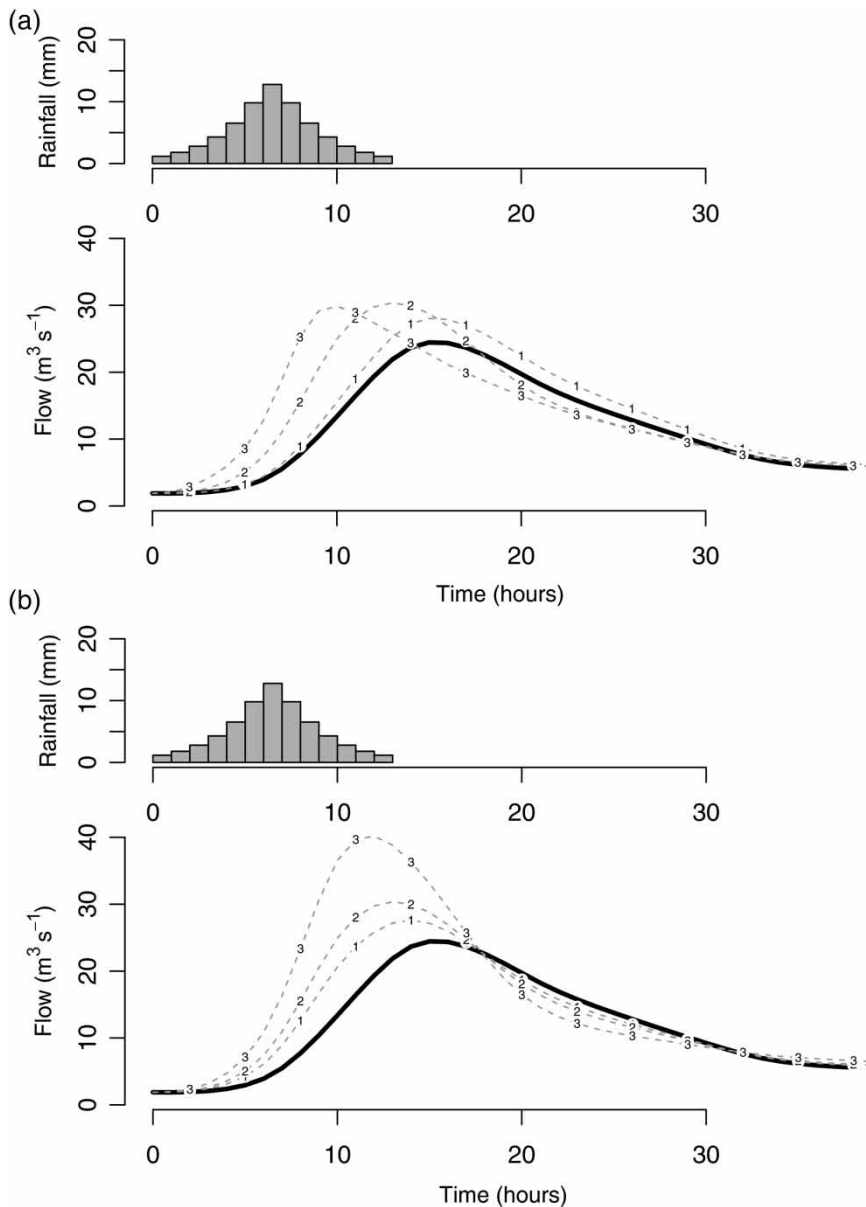
Figure 7 | Design flood hydrographs with a 100-year return period generated by the Rural model (black) and the Urban3 model for (a) URBEXT_{2000} = 0.200 and T_p ratio values of 1.0 (index 1), 0.5 (index 2) and 0.25 (index 3); and (b) T_p ratio of 0.50 and URBEXT_{2000} values of 0.125 (index 1), 0.20 (index 2) and 0.40 (index 3).
