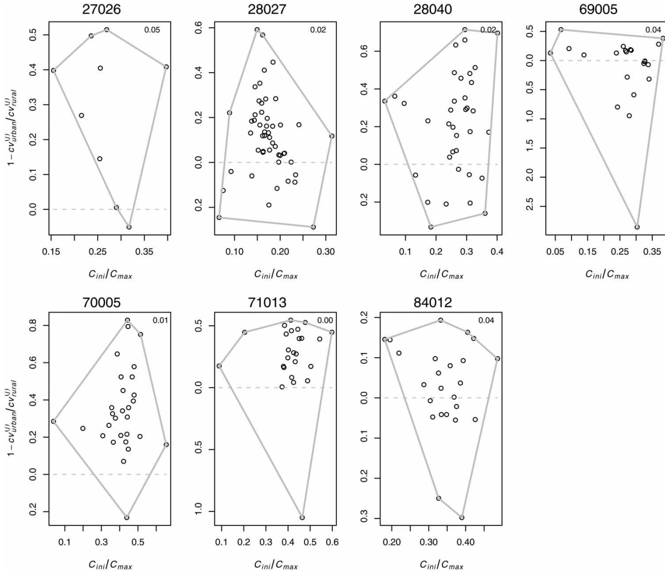
Figure 5 | Plot of relative cross-validation statistics (Equation (13), percentage improvement over original model) against initial soil moisture content C_{ini}/C_{max} for model Urban3. Number in upper right corner of each plot is the r^2 coefficient of determination value obtained through linear regression.
