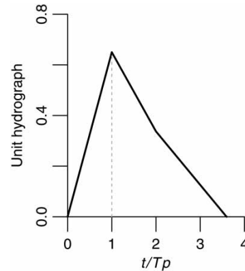
Figure 1 | Instantaneous unit hydrograph (IUH) of ReFH model.
