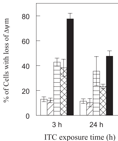
Figure 2. Effect of AITC or BITC on \Delta\Psi_m in HL60/S cells. Cells were exposed to vehicle (□), 2 μM AITC (▨), 10 μM AITC (▩), 2 μM BITC (▣), or 10 μM BITC (■) for 3 or 24 h. Cells then were harvested for determination of \Delta\Psi_m by flow cytometry. Columns, mean of three measurements; bars, SD. The values obtained from ITC-treated cells, except for 2 μM AITC, were significantly different from the values in the control cells ( t test, P < 0.01).
