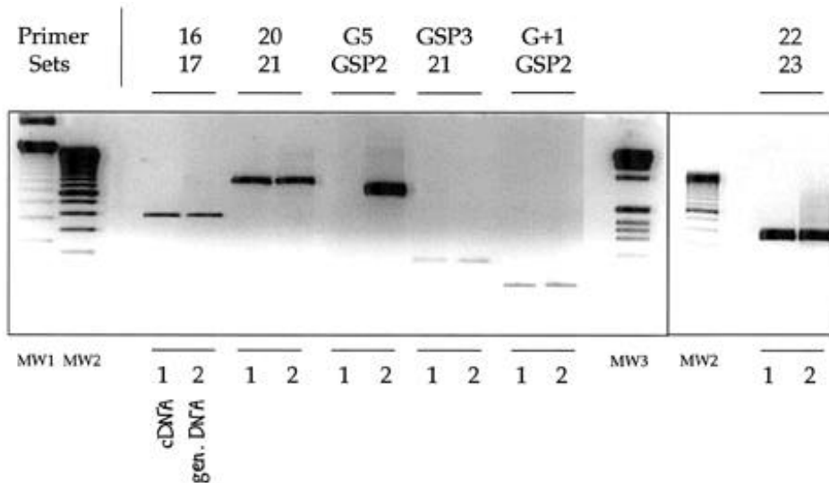
FIG. 2. \alpha -Endosulfine PCR amplified products generated with cDNA (1) and genomic DNA (2) templates. MW1, MW2, and MW3 represent 123-bp, 100-bp, and 1-kb ladders, respectively (Life Technologies molecular weight markers). Location of the primer sets used in PCR is indicated in Table 1.
