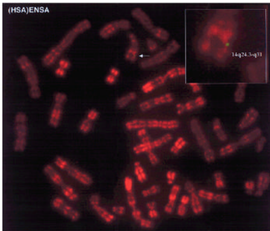
FIG. 3. Human metaphase chromosomes showing the specific hybridization of the \alpha -endosulfine probe to chromosome 14q24.3–q31 (indicated by the arrow).
