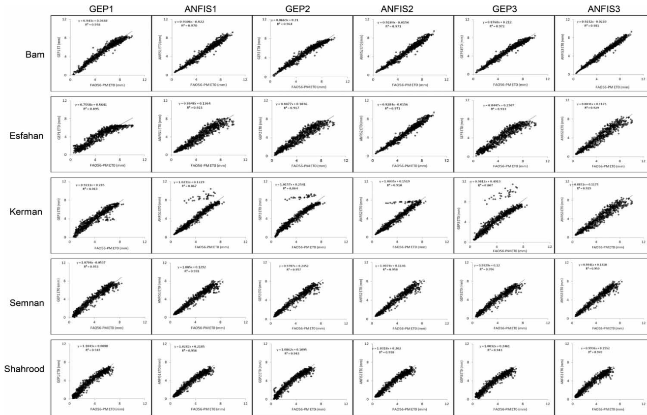
Figure 5 | Scatter plots of the applied models for pooled data approach (scenario 2).
