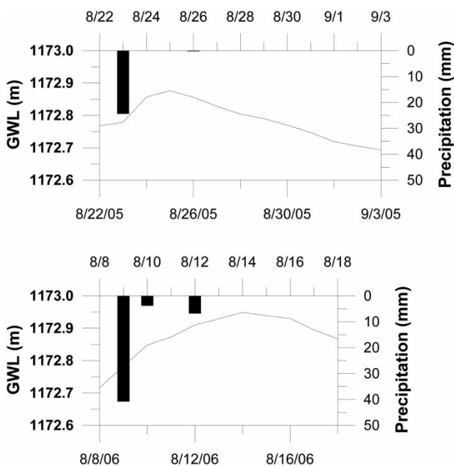
Figure 7 | Daily groundwater level (GWL) at G1 and daily precipitation. Since GWL is plotted as a daily value, diurnal fluctuations are not shown.
