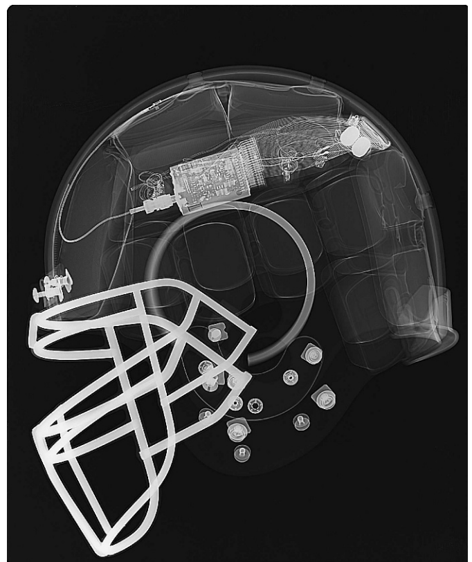
Figure 1. The Head Impact Telemetry System encoder placed within the padding of a football helmet around the crown of the head. (Photograph courtesy of Simbex LLC, Lebanon, NH.)
