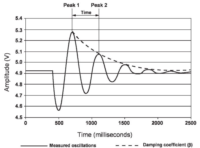
Figure 2. Stiffness calculation.
