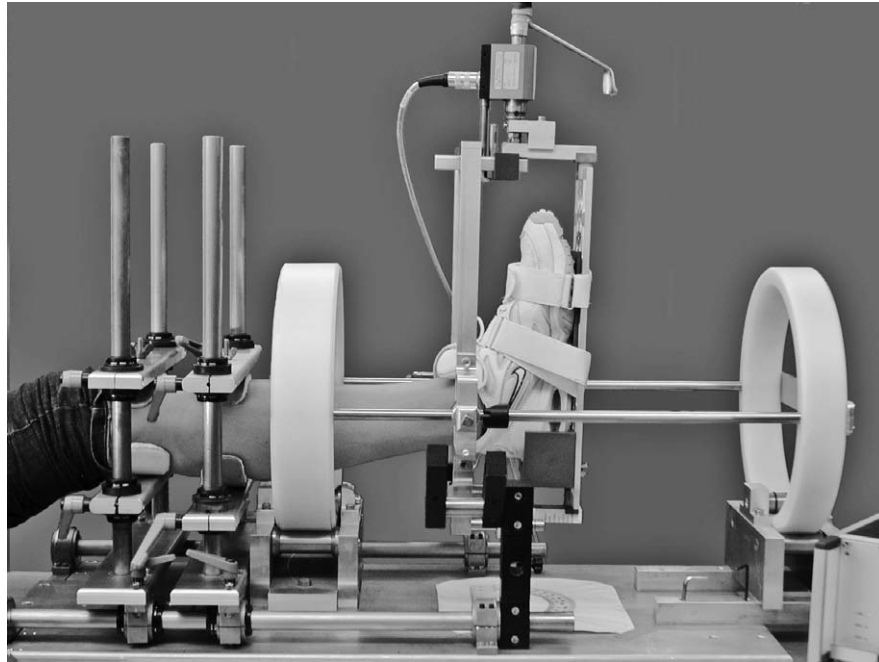
Figure 3. Apparatus for the measurement of maximal joint angles in 3 movement planes (6 directions) with an induced torque of 9 and 12 Nm only for dorsiflexion. Here, the unbraced condition is illustrated.
