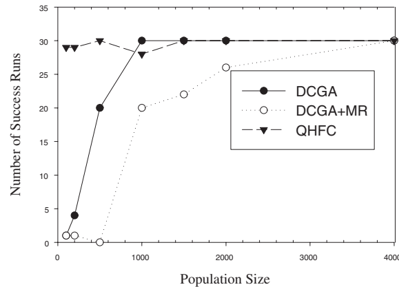
Figure 13: Comparison of QHFC with DCGA with/without multiple partial reinitializations in terms of robustness of the search capability and robustness in terms of population size. For the simple 128-bit HIFF problem, DCGA can achieve robust search if the population size is sufficiently large ( \geq 1000 ). QHFC, instead, can do very robust search from population sizes 100 to 4000. For the difficult 256-bit HIFF problem, a population size of 4000 for DCGA can only find the solution in half the 30 runs, while QHFC can solve it very robustly while still using population sizes from 100 to 4000. DCGA+MR apparently suffers from the disturbance of imported random individuals and works worse in both case than DCGA.
