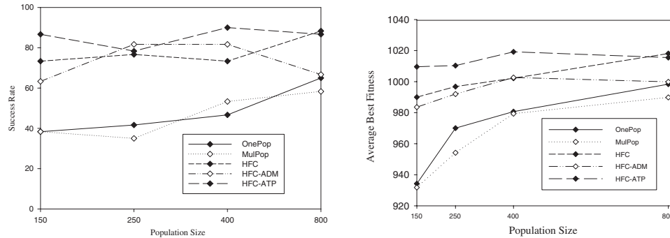
(a) Comparison of success rates after 300,000 evaluations: HFC techniques consistently outperform standard OnePop and MulPop GP and are essentially invariant with respect to population size.
