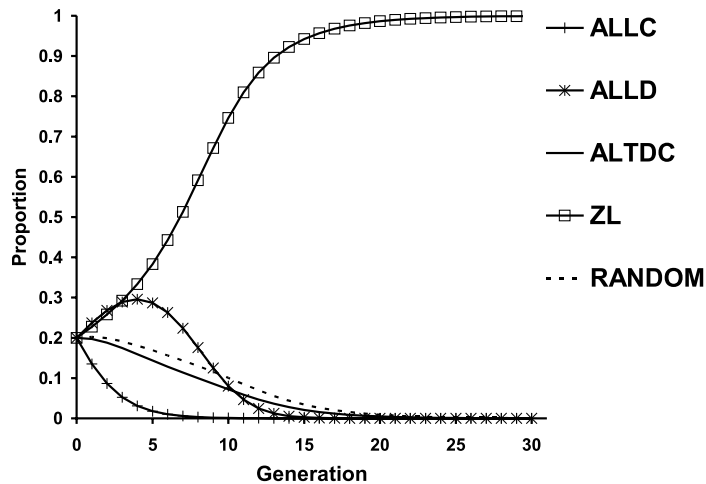
Figure 6. ZL and group 1 schemes in the EPD for pr = 0 . In few generations, ZL reached 100% of the population.
