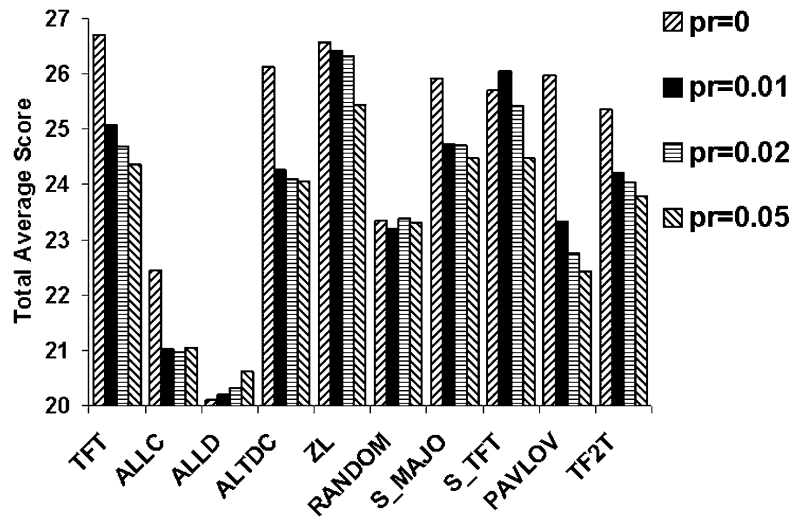
Figure 4. Total average score for each strategy and probability of random moves. TFT obtained the highest score for pr = 0 , followed closely by ZL. For the other pr s, ZL was the best strategy. Its performance was not significantly affected by pr .
