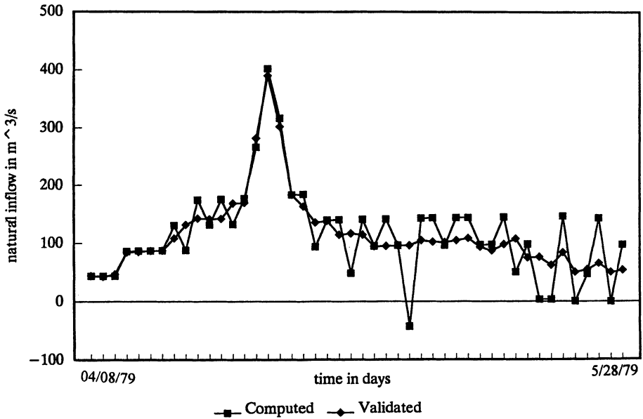
Fig. 10. Comparison between computed and validated natural inflows based on gauge 32312005.
