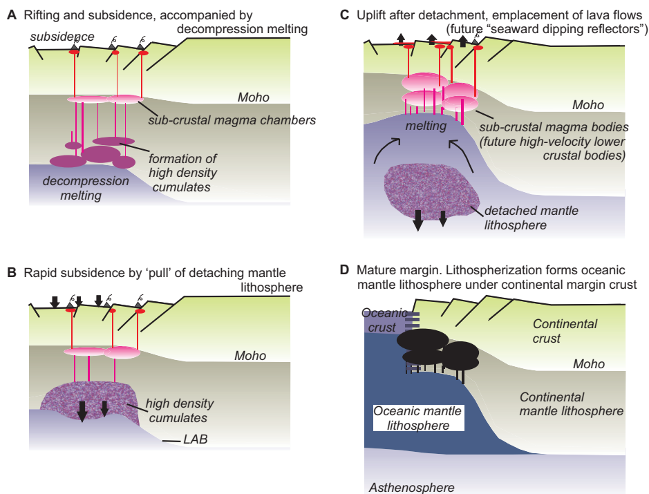
Figure 4. Conceptual model of rifted margin formation. (A) Decompression melting of upwelling asthenosphere accompanies lithosphere thinning during continental rifting. Magmatic differentiation in the lithosphere results in the formation of high-density cumulates. (B) The high-density cumulates destabilize the mantle lithosphere. This results in extra subsidence of the rifted area during detachment. LAB—lithosphere-asthenosphere boundary. (C) After detachment, the surface is uplifted while melting continues, followed by continental rupture. Sub-Moho intrusions are future fast seismic wave velocity lower crustal bodies, lava flows are emplaced at the surface. At magma-poor margins there are no (or few) magmatic eruptions at this time. (D) Following continental breakup, lithospherization of upwelled asthenosphere below the margin occurs.
