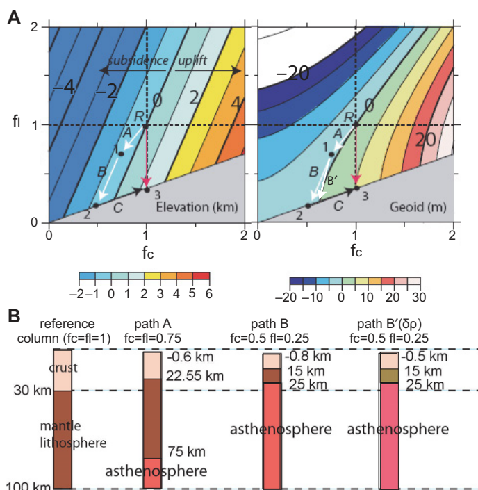
Figure 3. Isostatic diagrams to illustrate the effects of depth-dependent thinning and lithospheric modification on the isostatic response of the lithosphere, and predicted geoid anomalies; f_c is crustal thinning, f_l is lithosphere thinning (calculated as percent strain). Values <1 indicate thinning. Units on the color bar are elevation (in km; left panel) and geoid (in m; right panel). Points 1, 2, and 3 are end points of the different paths. (A) Surface elevation changes in response to crustal and lithospheric thickness variations. Right panel: geoid anomaly (see Coblenz et al., 2011, and text for description of how this geoid is calculated). The arrows (paths) show the uplift and subsidence trends. R is the starting point (undisturbed lithosphere); the red arrow connects the starting and end points. (B) Isostatic columns corresponding to paths A, B, and B'. B' is a modification of path B, including density variations due to phase transitions. In path B' the density of the entire mantle lithosphere has been decreased by 2.3%. See text for further explanation.
