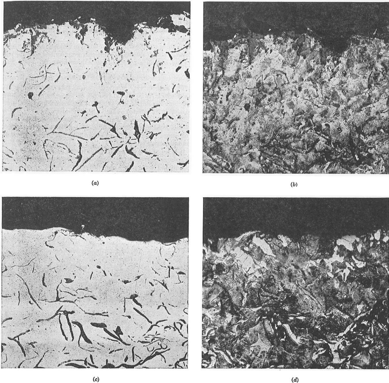
FIG. 9 PHOTOMICROGRAPHS OF CAST SURFACES; \times 100 (a, Unetched tumbled surface reveals rough decarburized surface. b, Etched tumbled surface reveals pearlitic structure. c, Unetched shot-blasted surface. Shot-blasting produces a smoother surface than tumbling. d, Etched shot-blasted surface shows pearlite and ferrite.)
