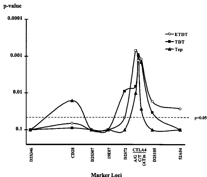
FIG. 2. Association of markers on chromosome 2q33 with IDDM. The P values for the TDT, ETDT, and Tsp analyses of each marker are plotted against the approximate distance of the markers. When the P values are >0.1 , they are plotted at the 0.1 position. A peak of linkage and association was observed in the CTLA4 region.
