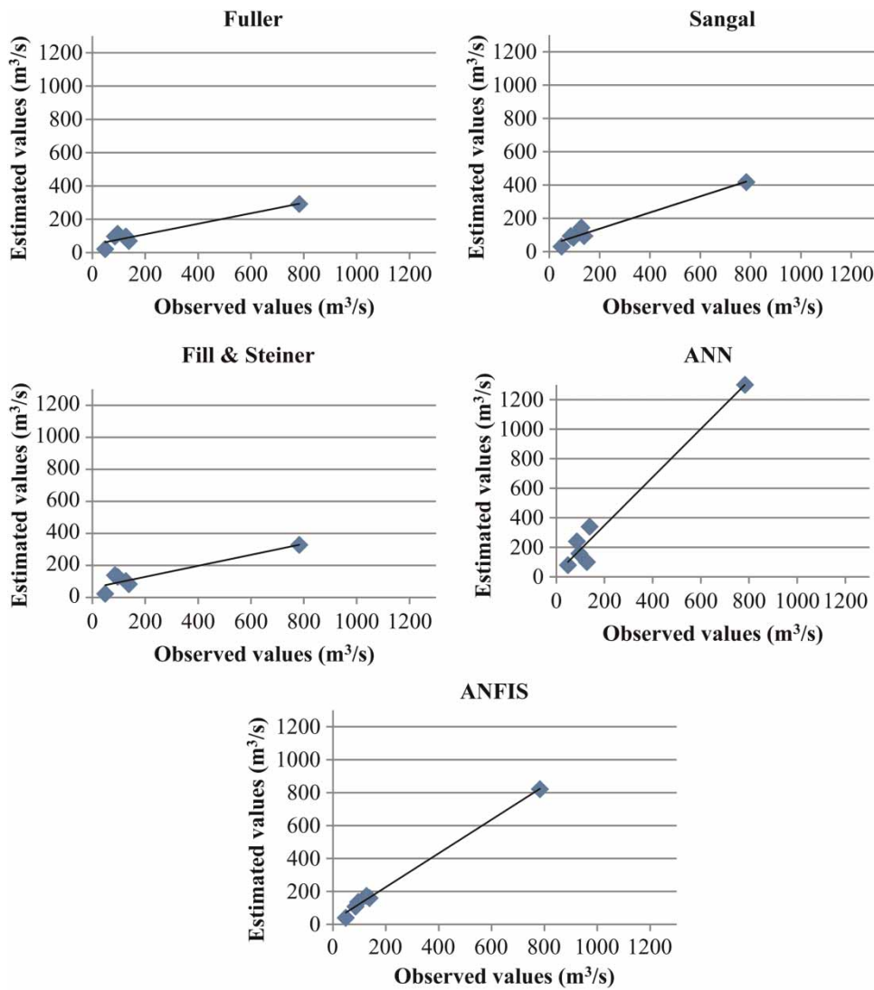
Figure 4 | Instantaneous peak flow estimated by different methods versus the observed values in gauging station code 12-005.
