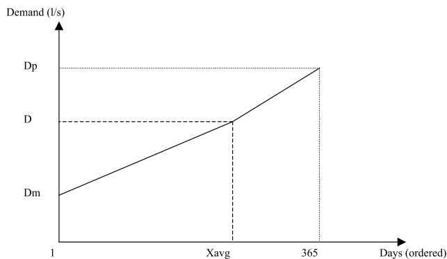
Figure 4 | Classified curve of daily needs.
