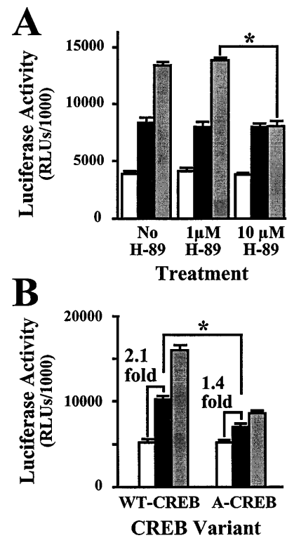
FIG. 5. A: PKA antagonist H-89 produced a concentration-dependent inhibition of 2 \mu\text{mol/l} forskolin-stimulated -410\text{RIP1-LUC} activity in transfected INS-1 cells. H-89 did not inhibit luciferase activity stimulated by 10 nmol/l GLP-1 (7-37). *P \leq 0.001 . B: Transfection with dominant-negative A-CREB reduced 10 nmol/l GLP-1 (7-37)-stimulated luciferase activity in cells cotransfected with -410\text{RIP1-LUC} . A-CREB was also an effective antagonist of 2 \mu\text{mol/l} forskolin-stimulated luciferase activity. *P \leq 0.01 . \square , Basal; \blacksquare , GLP-1; \square , forskolin.
