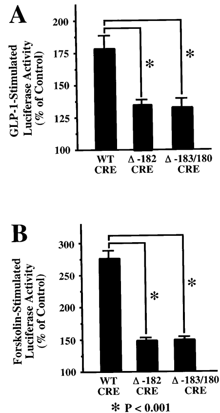
FIG. 8. A: Single-base pair ( \Delta-182 ) or 4-base pair ( \Delta-183/180 ) deletions of the RIP1 CRE reduced 10 nmol/l GLP-1 (7-37)-stimulated luciferase activity in INS-1 cells transfected with -410\text{RIP1-LUC} . B: The stimulatory action of 2 \mu\text{mol/l} forskolin was also reduced by introduction of \Delta-182 or \Delta-183/180 deletions of the RIP1 CRE.
