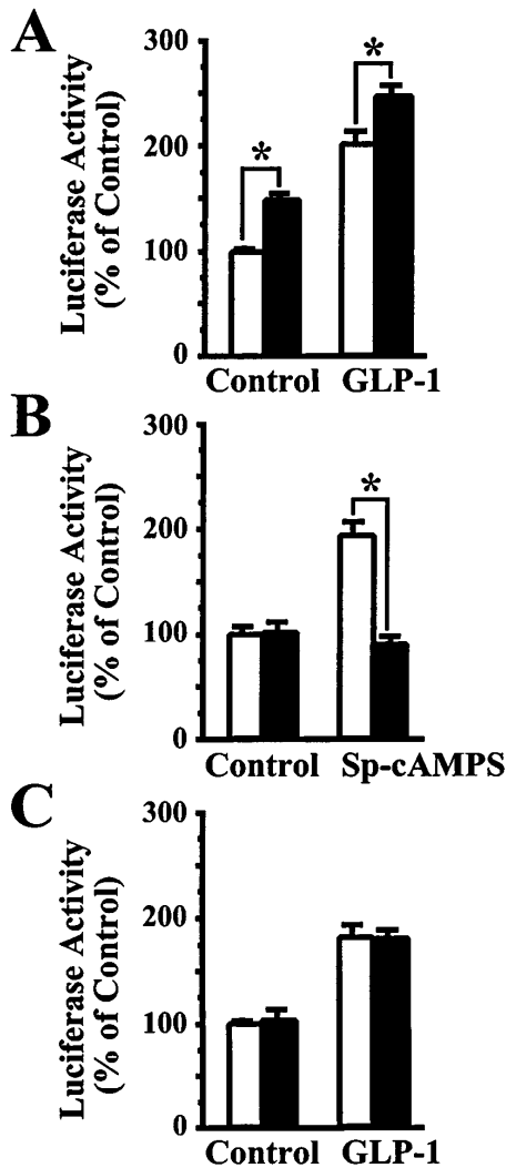
FIG. 4. A: Sp-cAMPS (50 \mu\text{mol/l} ) stimulated -410\text{RIP1-LUC} activity in INS-1 cellular lysates. The action of Sp-cAMPS was potentiated by 10 nmol/l GLP-1 (7-37). \square , No Sp-cAMPS; \blacksquare , 50 \mu\text{mol/l} Sp-cAMPS; *P \leq 0.05 . B: Rp-cAMPS (50 \mu\text{mol/l} ) blocked stimulation of -410\text{RIP1-LUC} by 50 \mu\text{mol/l} Sp-cAMPS. \square , No Rp-cAMPS; \blacksquare , 50 \mu\text{mol/l} Rp-cAMPS; *P \leq 0.001 . C: Failure of 50 \mu\text{mol/l} Rp-cAMPS to block stimulation of -410\text{RIP1-LUC} by 10 nmol/l GLP-1 (7-37). \square , No Rp-cAMPS; \blacksquare , 50 \mu\text{mol/l} Rp-cAMPS. Values of luciferase activity are expressed as the percentage of control.
