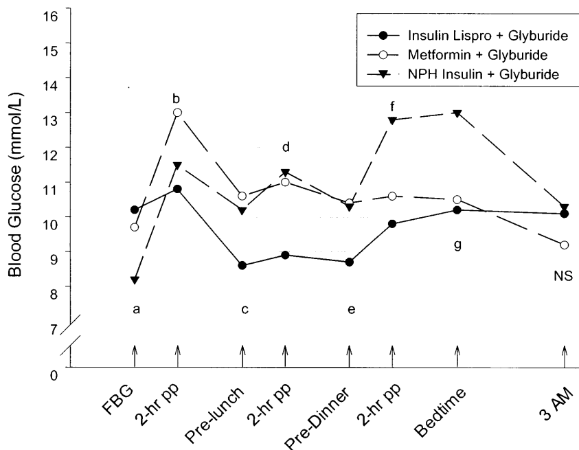
Figure 2 —An 8-point blood glucose profile as determined from home blood glucose monitoring. Curves represent endpoint mean blood glucose values for the 3 groups (the means of 8-point blood glucose profiles performed 3 days and 1 day before the final visit). 2-hr pp, 2-h postprandial; a, NPH+G vs. M+G ( P = 0.015 ) or L+G ( P = 0.001 ); b, L+G vs. M+G ( P = 0.009 ); c, L+G vs. M+G ( P = 0.006 ) or NPH+G ( P = 0.030 ); d, L+G vs. M+G ( P = 0.007 ) or NPH+G ( P = 0.002 ); e, L+G vs. M+G ( P = 0.033 ) or NPH+G ( P = 0.039 ); f, L+G or M+G vs. NPH+G ( P < 0.01 for both comparisons); g, L+G or M+G vs. NPH+G ( P < 0.01 for both comparisons).
